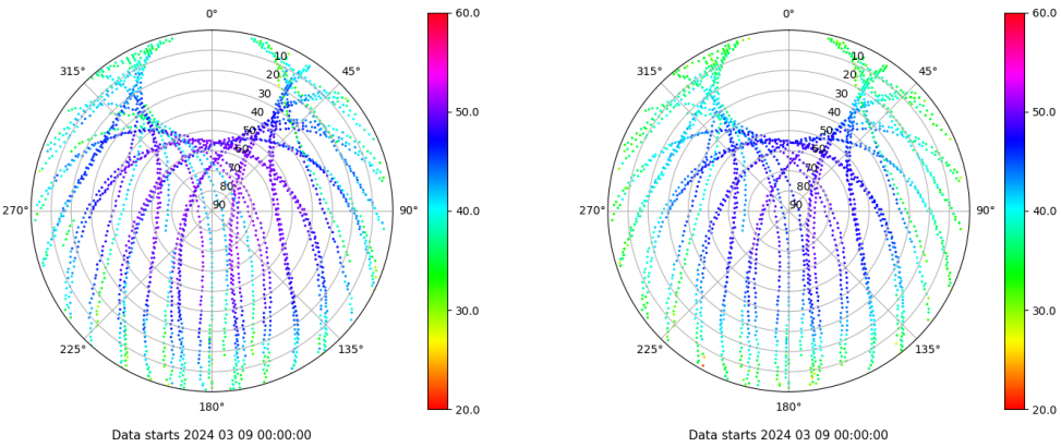
Skyplot for station IBIZ. Signal to Noise S1C Data file IBIZ00ESP_R_2024069.xtr Skyplot for station IBIZ. Signal to Noise S2P Data file IBIZ00ESP_R_2024069.xtr
