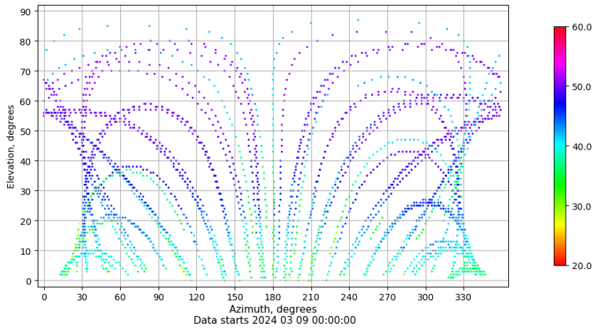
Azimuth-elevation plot for station IBIZ. Signal to Noise S1C Data file IBIZ00ESP_R_2024069.xtr
