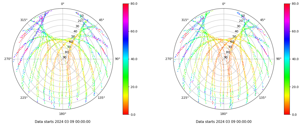
Skyplot for station IBIZ. Parameter M1C Data file IBIZ00ESP_R_2024069.xtr Skyplot for station IBIZ. Parameter M2P Data file IBIZ00ESP_R_2024069.xtr
