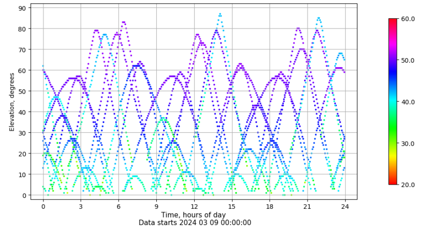
Time-elevation plot for station IBIZ. Signal to Noise S1C Data file IBIZ00ESP_R_2024069.xtr
