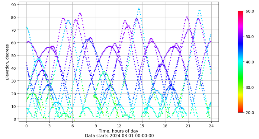
Time-elevation plot for station IBIZ. Signal to Noise S1C Data file IBIZ00ESP_R_2024061.xtr
