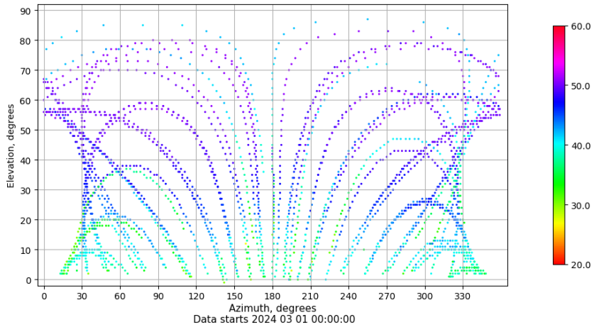
Azimuth-elevation plot for station IBIZ. Signal to Noise S1C Data file IBIZ00ESP_R_2024061.xtr
