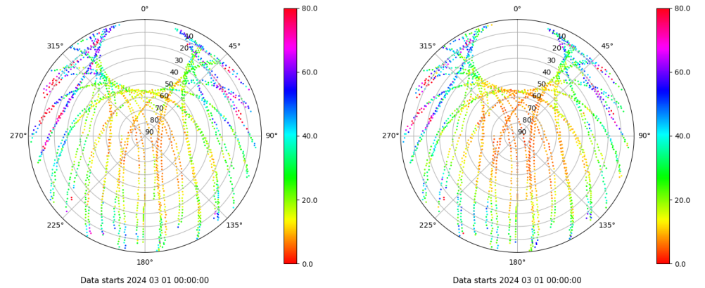
Skyplot for station IBIZ. Parameter M1C Data file IBIZ00ESP_R_2024061.xtr Skyplot for station IBIZ. Parameter M2P Data file IBIZ00ESP_R_2024061.xtr
