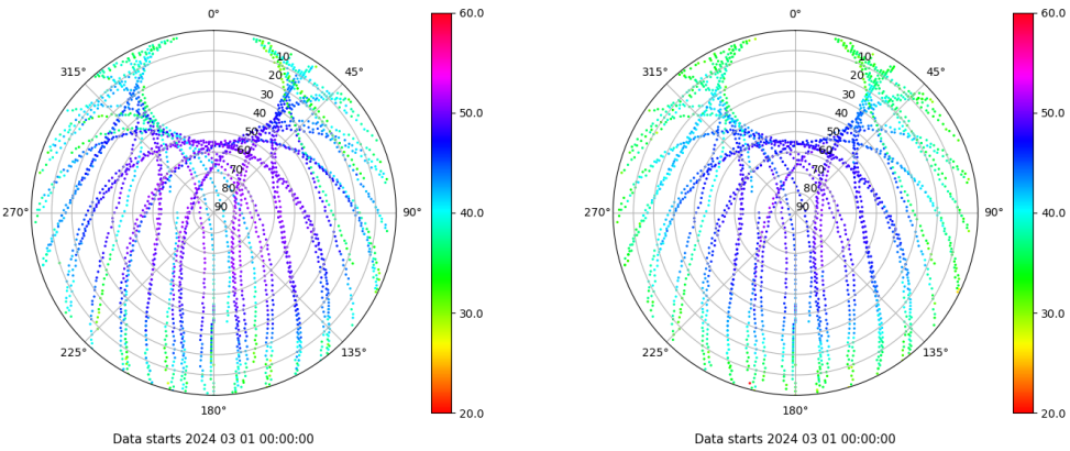
Skyplot for station IBIZ. Signal to Noise S1C Data file IBIZ00ESP_R_2024061.xtr Skyplot for station IBIZ. Signal to Noise S2P Data file IBIZ00ESP_R_2024061.xtr
