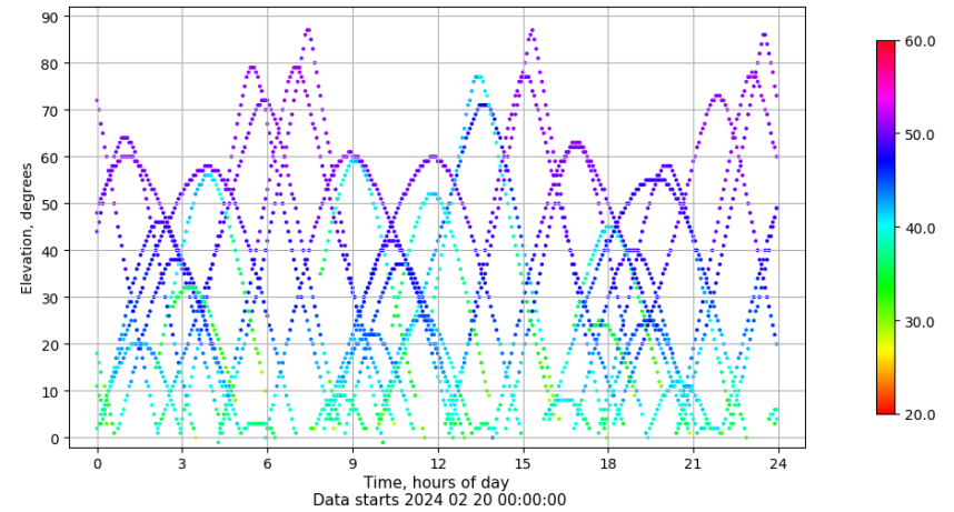
Time-elevation plot for station IBIZ. Signal to Noise S1C Data file IBIZ00ESP_R_2024051.xtr
