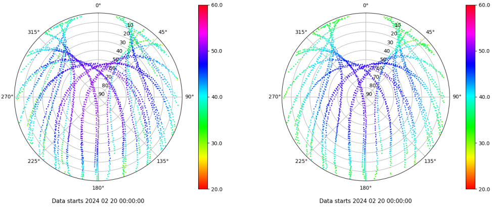
Skyplot for station IBIZ. Signal to Noise S1C Data file IBIZ00ESP_R_2024051.xtr Skyplot for station IBIZ. Signal to Noise S2P Data file IBIZ00ESP_R_2024051.xtr
