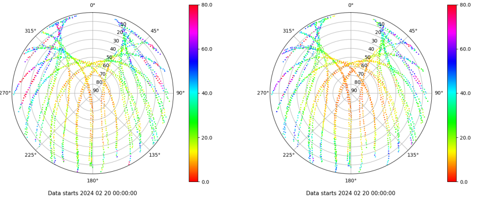
Skyplot for station IBIZ. Parameter M1C Data file IBIZ00ESP_R_2024051.xtr Skyplot for station IBIZ. Parameter M2P Data file IBIZ00ESP_R_2024051.xtr
