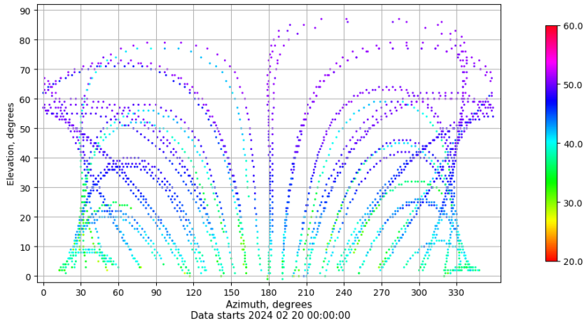
Azimuth-elevation plot for station IBIZ. Signal to Noise S1C Data file IBIZ00ESP_R_2024051.xtr
