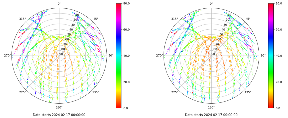
Skyplot for station IBIZ. Parameter M1C Data file IBIZ00ESP_R_2024048.xtr Skyplot for station IBIZ. Parameter M2P Data file IBIZ00ESP_R_2024048.xtr
