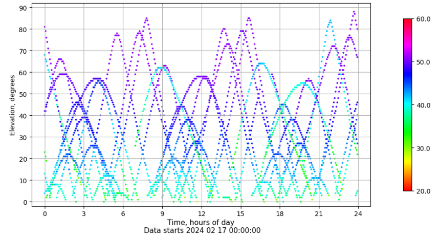
Time-elevation plot for station IBIZ. Signal to Noise S1C Data file IBIZ00ESP_R_2024048.xtr
