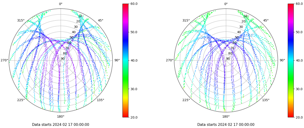
Skyplot for station IBIZ. Signal to Noise S1C Data file IBIZ00ESP_R_2024048.xtr Skyplot for station IBIZ. Signal to Noise S2P Data file IBIZ00ESP_R_2024048.xtr
