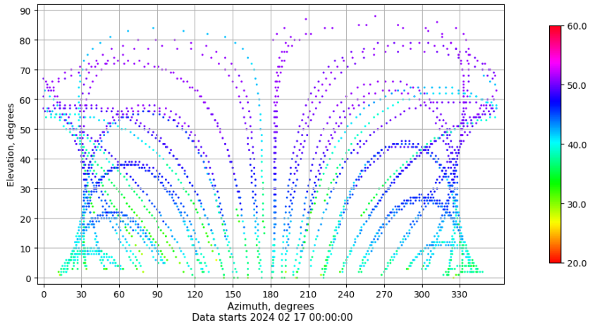
Azimuth-elevation plot for station IBIZ. Signal to Noise S1C Data file IBIZ00ESP_R_2024048.xtr
