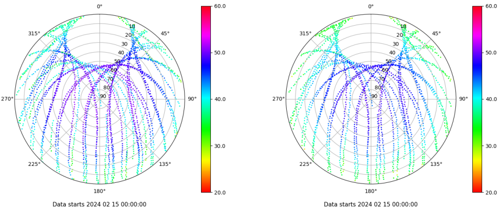
Skyplot for station IBIZ. Signal to Noise S1C Data file IBIZ00ESP_R_2024046.xtr Skyplot for station IBIZ. Signal to Noise S2P Data file IBIZ00ESP_R_2024046.xtr
