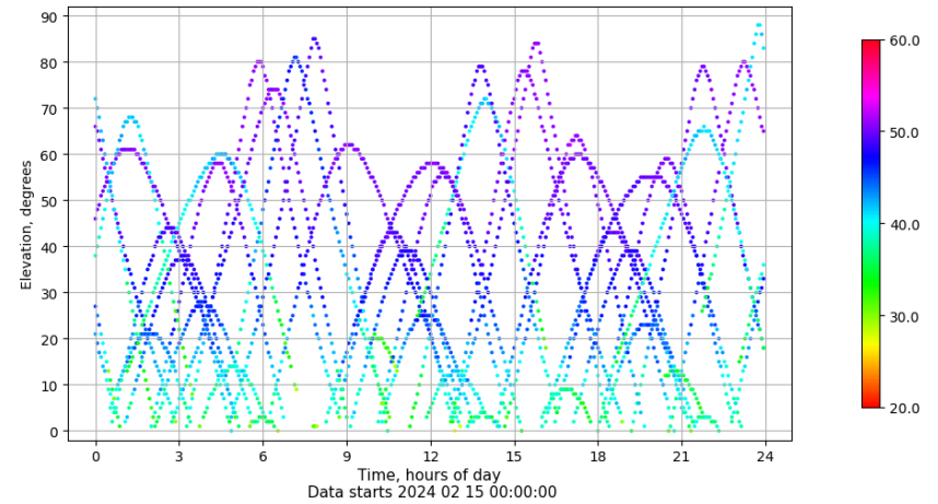
Time-elevation plot for station IBIZ. Signal to Noise S1C Data file IBIZ00ESP_R_2024046.xtr
