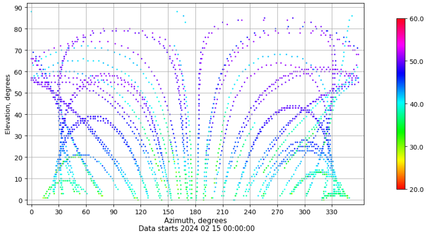
Azimuth-elevation plot for station IBIZ. Signal to Noise S1C Data file IBIZ00ESP_R_2024046.xtr
