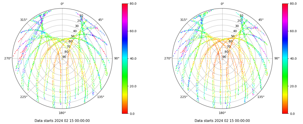
Skyplot for station IBIZ. Parameter M1C Data file IBIZ00ESP_R_2024046.xtr Skyplot for station IBIZ. Parameter M2P Data file IBIZ00ESP_R_2024046.xtr
