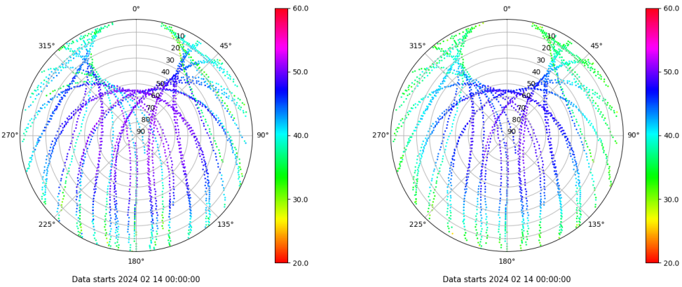
Skyplot for station IBIZ. Signal to Noise S1C Data file IBIZ00ESP_R_2024045.xtr Skyplot for station IBIZ. Signal to Noise S2P Data file IBIZ00ESP_R_2024045.xtr
