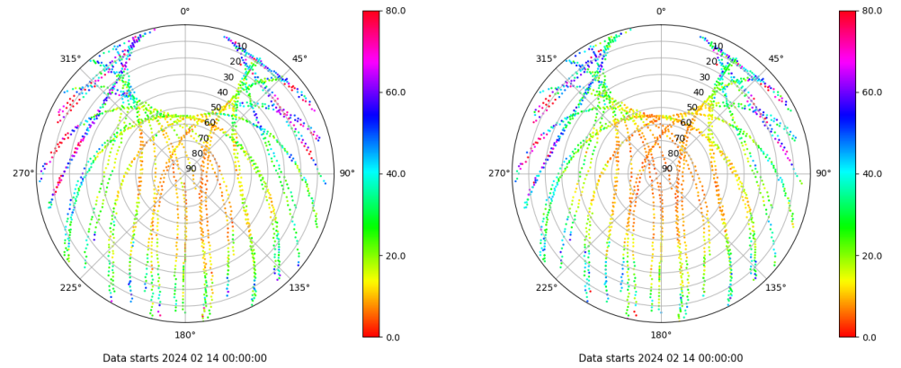
Skyplot for station IBIZ. Parameter M1C Data file IBIZ00ESP_R_2024045.xtr Skyplot for station IBIZ. Parameter M2P Data file IBIZ00ESP_R_2024045.xtr
