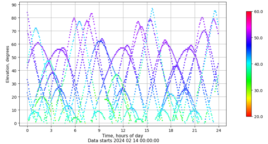
Time-elevation plot for station IBIZ. Signal to Noise S1C Data file IBIZ00ESP_R_2024045.xtr
