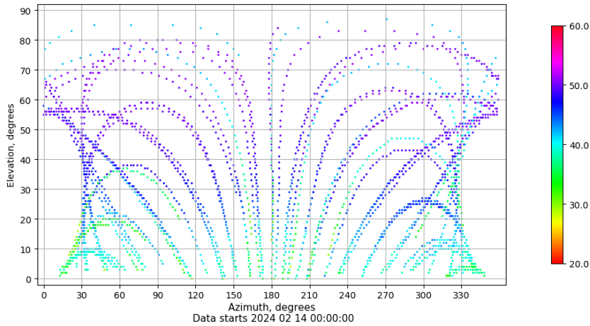
Azimuth-elevation plot for station IBIZ. Signal to Noise S1C Data file IBIZ00ESP_R_2024045.xtr
