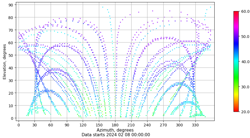
Azimuth-elevation plot for station IBIZ. Signal to Noise S1C Data file IBIZ00ESP_R_2024039.xtr
