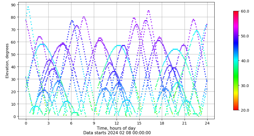
Time-elevation plot for station IBIZ. Signal to Noise S1C Data file IBIZ00ESP_R_2024039.xtr
