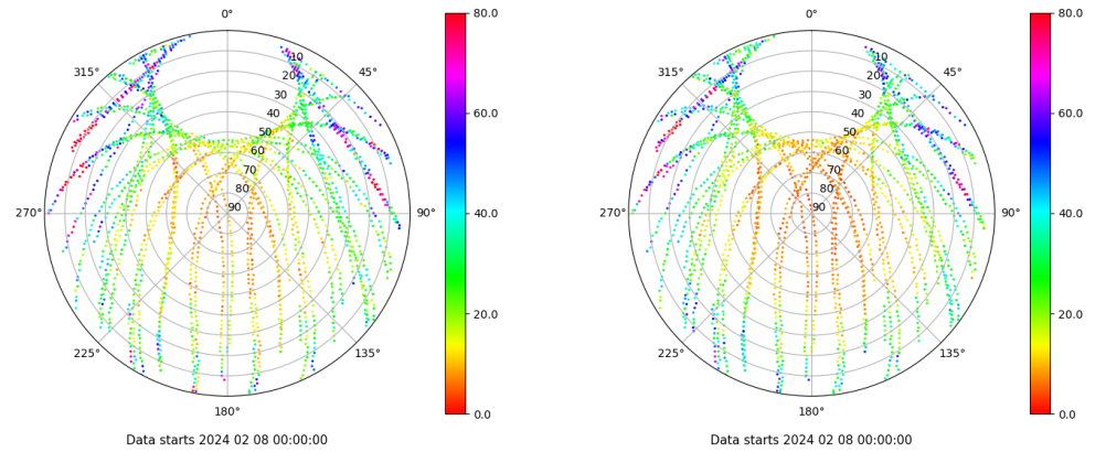
Skyplot for station IBIZ. Parameter M1C Data file IBIZ00ESP_R_2024039.xtr Skyplot for station IBIZ. Parameter M2P Data file IBIZ00ESP_R_2024039.xtr
