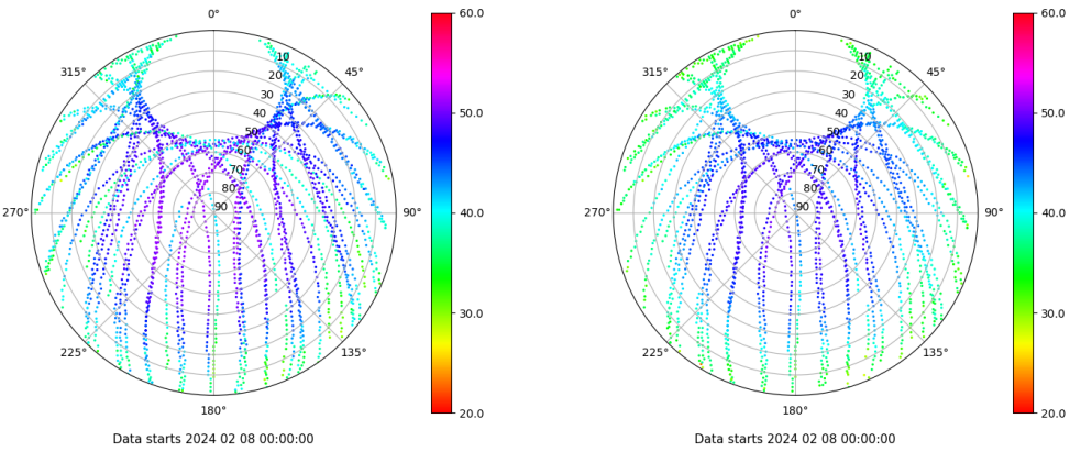
Skyplot for station IBIZ. Signal to Noise S1C Data file IBIZ00ESP_R_2024039.xtr Skyplot for station IBIZ. Signal to Noise S2P Data file IBIZ00ESP_R_2024039.xtr
