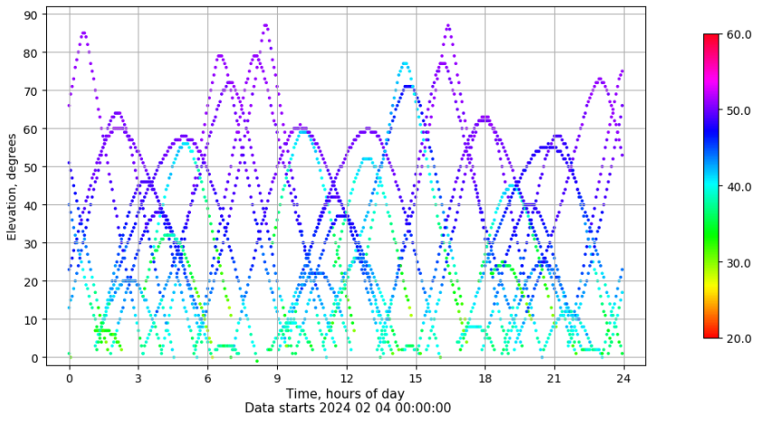
Time-elevation plot for station IBIZ. Signal to Noise S1C Data file IBIZ00ESP_R_2024035.xtr
