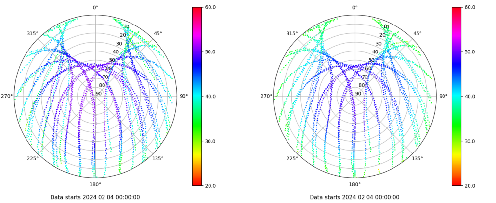
Skyplot for station IBIZ. Signal to Noise S1C Data file IBIZ00ESP_R_2024035.xtr Skyplot for station IBIZ. Signal to Noise S2P Data file IBIZ00ESP_R_2024035.xtr
