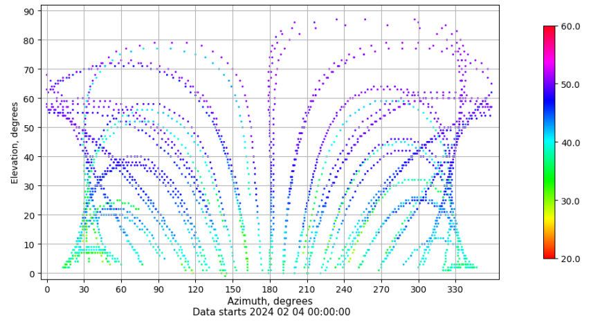
Azimuth-elevation plot for station IBIZ. Signal to Noise S1C Data file IBIZ00ESP_R_2024035.xtr
