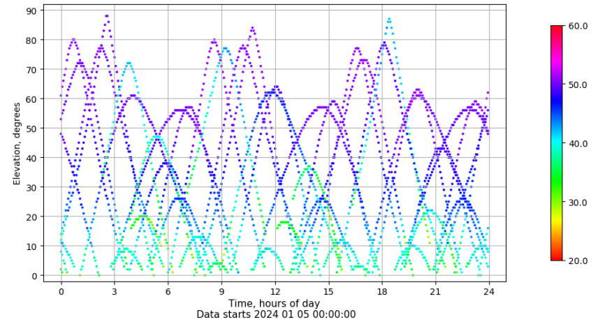
Time-elevation plot for station IBIZ. Signal to Noise S1C Data file IBIZ00ESP_R_2024005.xtr
