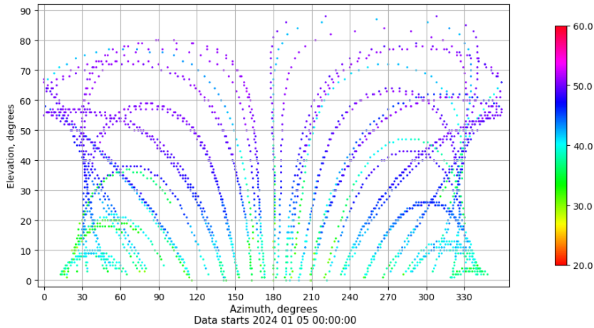
Azimuth-elevation plot for station IBIZ. Signal to Noise S1C Data file IBIZ00ESP_R_2024005.xtr
