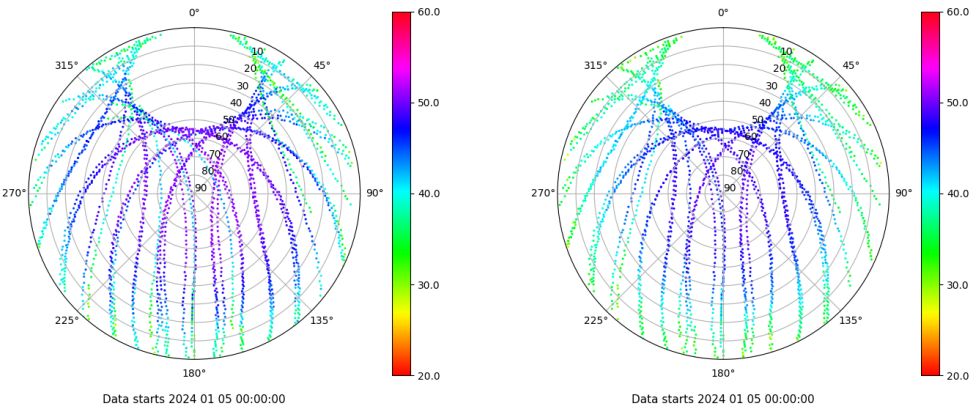
Skyplot for station IBIZ. Signal to Noise S1C Data file IBIZ00ESP_R_2024005.xtr Skyplot for station IBIZ. Signal to Noise S2P Data file IBIZ00ESP_R_2024005.xtr
