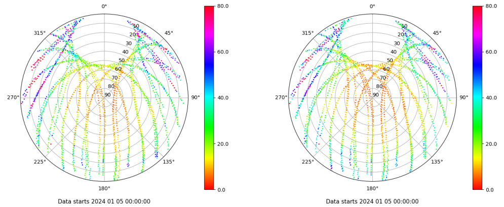
Skyplot for station IBIZ. Parameter M1C Data file IBIZ00ESP_R_2024005.xtr Skyplot for station IBIZ. Parameter M2P Data file IBIZ00ESP_R_2024005.xtr
