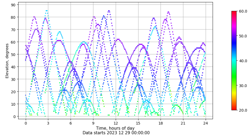
Time-elevation plot for station IBIZ. Signal to Noise S1C Data file IBIZ00ESP_R_2023363.xtr
