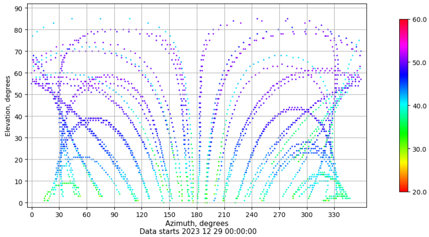
Azimuth-elevation plot for station IBIZ. Signal to Noise S1C Data file IBIZ00ESP_R_2023363.xtr
