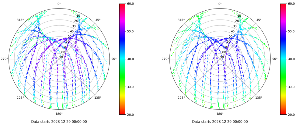
Skyplot for station IBIZ. Signal to Noise S1C Data file IBIZ00ESP_R_2023363.xtr Skyplot for station IBIZ. Signal to Noise S2P Data file IBIZ00ESP_R_2023363.xtr
