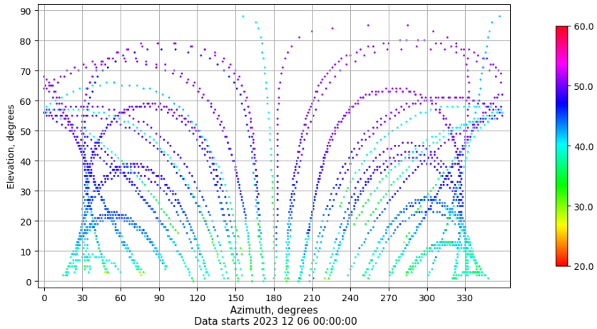
Azimuth-elevation plot for station IBIZ. Signal to Noise S1C Data file IBIZ00ESP_R_2023340.xtr
