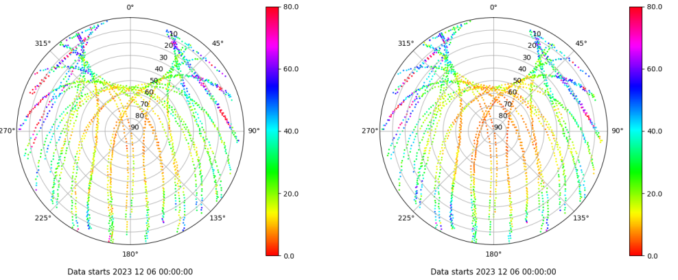
Skyplot for station IBIZ. Parameter M1C Data file IBIZ00ESP_R_2023340.xtr Skyplot for station IBIZ. Parameter M2P Data file IBIZ00ESP_R_2023340.xtr
