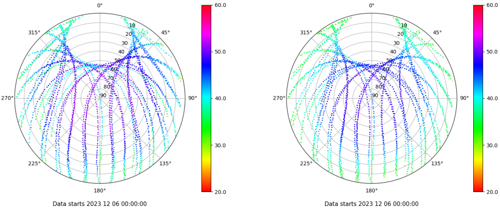
Skyplot for station IBIZ. Signal to Noise S1C Data file IBIZ00ESP_R_2023340.xtr Skyplot for station IBIZ. Signal to Noise S2P Data file IBIZ00ESP_R_2023340.xtr
