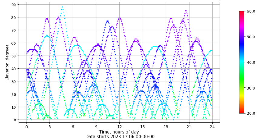
Time-elevation plot for station IBIZ. Signal to Noise S1C Data file IBIZ00ESP_R_2023340.xtr
