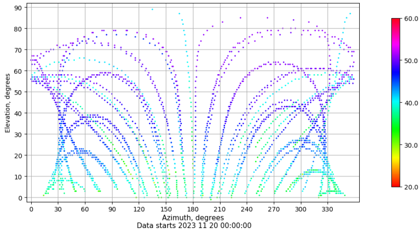
Azimuth-elevation plot for station IBIZ. Signal to Noise S1C Data file IBIZ00ESP_R_2023324.xtr
