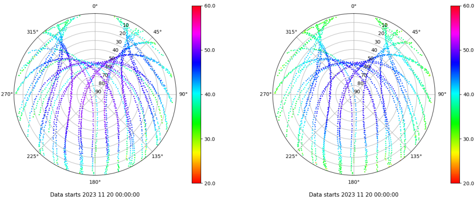
Skyplot for station IBIZ. Signal to Noise S1C Data file IBIZ00ESP_R_2023324.xtr Skyplot for station IBIZ. Signal to Noise S2P Data file IBIZ00ESP_R_2023324.xtr
