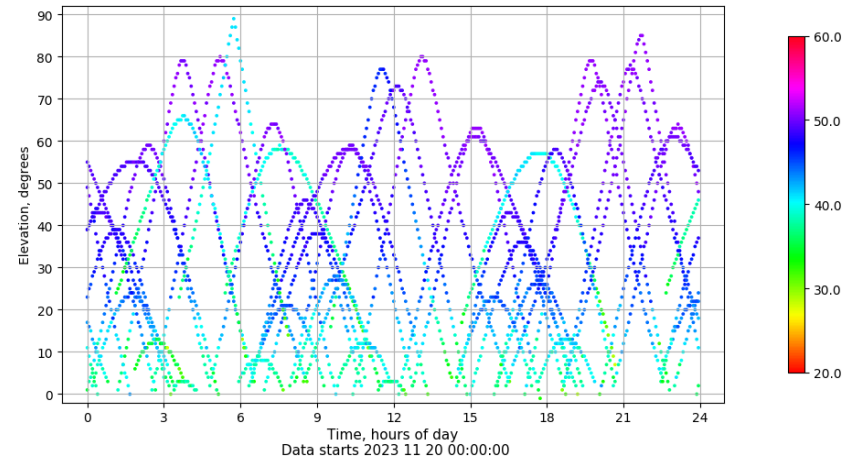
Time-elevation plot for station IBIZ. Signal to Noise S1C Data file IBIZ00ESP_R_2023324.xtr
