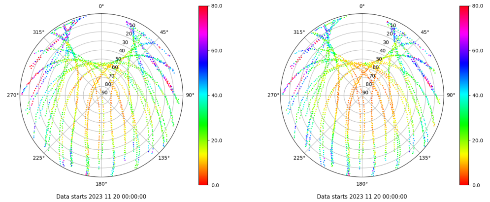
Skyplot for station IBIZ. Parameter M1C Data file IBIZ00ESP_R_2023324.xtr Skyplot for station IBIZ. Parameter M2P Data file IBIZ00ESP_R_2023324.xtr
