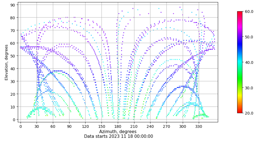
Azimuth-elevation plot for station IBIZ. Signal to Noise S1C Data file IBIZ00ESP_R_2023322.xtr
