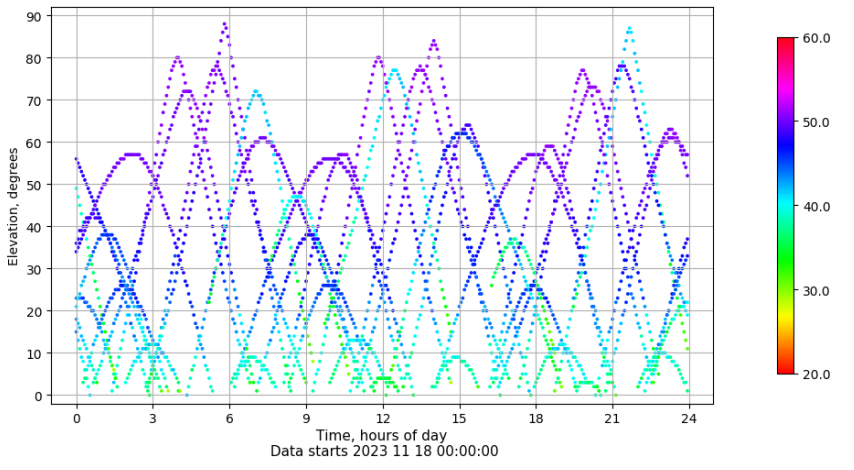
Time-elevation plot for station IBIZ. Signal to Noise S1C Data file IBIZ00ESP_R_2023322.xtr
