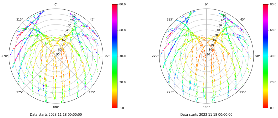
Skyplot for station IBIZ. Parameter M1C Data file IBIZ00ESP_R_2023322.xtr Skyplot for station IBIZ. Parameter M2P Data file IBIZ00ESP_R_2023322.xtr
