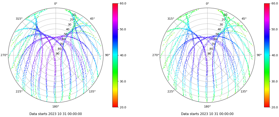
Skyplot for station IBIZ. Signal to Noise S1C Data file IBIZ00ESP_R_2023304.xtr Skyplot for station IBIZ. Signal to Noise S2P Data file IBIZ00ESP_R_2023304.xtr
