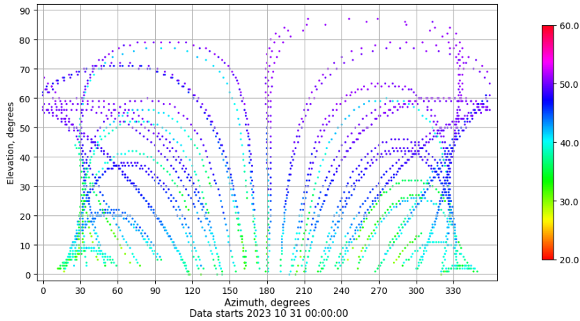
Azimuth-elevation plot for station IBIZ. Signal to Noise S1C Data file IBIZ00ESP_R_2023304.xtr
