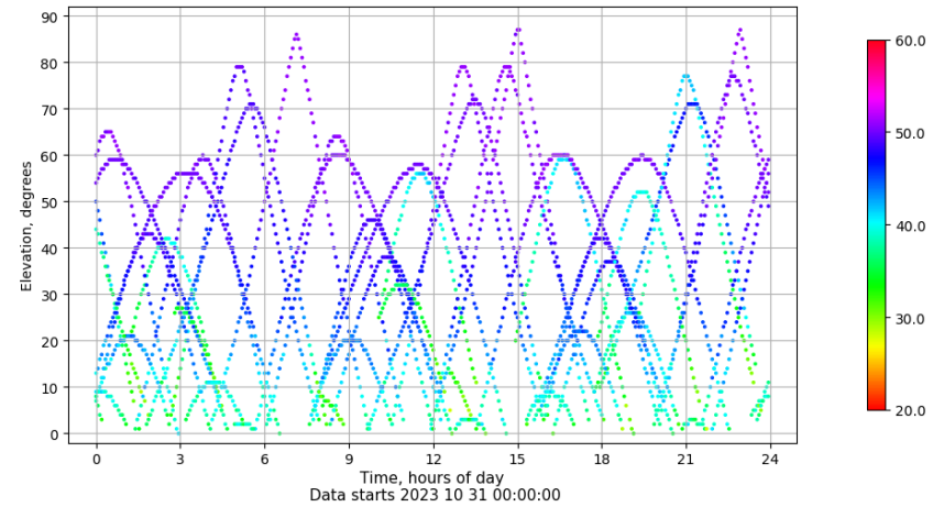
Time-elevation plot for station IBIZ. Signal to Noise S1C Data file IBIZ00ESP_R_2023304.xtr
