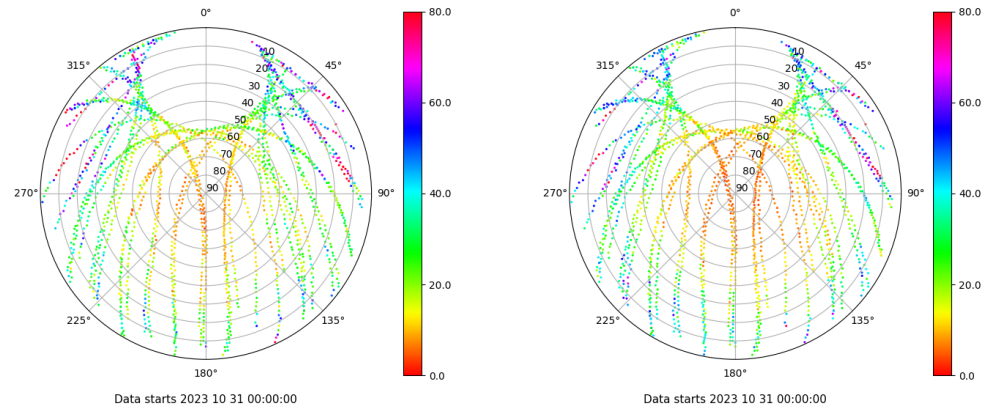
Skyplot for station IBIZ. Parameter M1C Data file IBIZ00ESP_R_2023304.xtr Skyplot for station IBIZ. Parameter M2P Data file IBIZ00ESP_R_2023304.xtr
