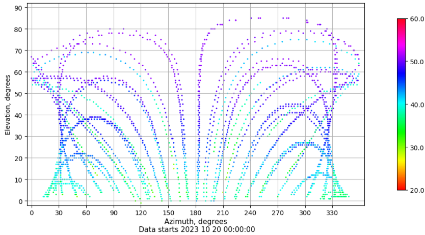
Azimuth-elevation plot for station IBIZ. Signal to Noise S1C Data file IBIZ00ESP_R_2023293.xtr
