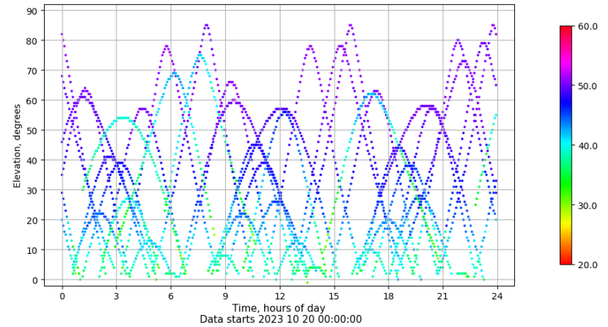
Time-elevation plot for station IBIZ. Signal to Noise S1C Data file IBIZ00ESP_R_2023293.xtr
