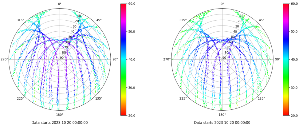
Skyplot for station IBIZ. Signal to Noise S1C Data file IBIZ00ESP_R_2023293.xtr Skyplot for station IBIZ. Signal to Noise S2P Data file IBIZ00ESP_R_2023293.xtr
