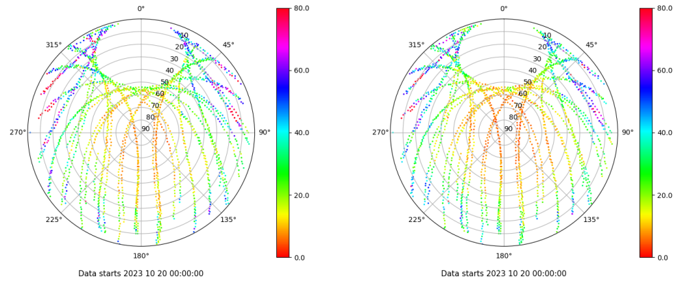
Skyplot for station IBIZ. Parameter M1C Data file IBIZ00ESP_R_2023293.xtr Skyplot for station IBIZ. Parameter M2P Data file IBIZ00ESP_R_2023293.xtr
