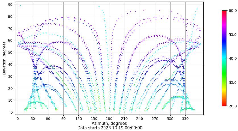
Azimuth-elevation plot for station IBIZ. Signal to Noise S1C Data file IBIZ00ESP_R_2023292.xtr
