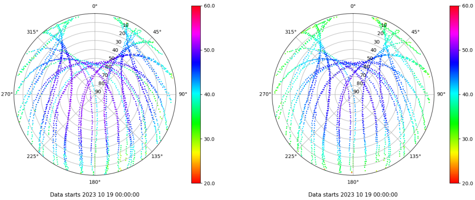
Skyplot for station IBIZ. Signal to Noise S1C Data file IBIZ00ESP_R_2023292.xtr Skyplot for station IBIZ. Signal to Noise S2P Data file IBIZ00ESP_R_2023292.xtr
