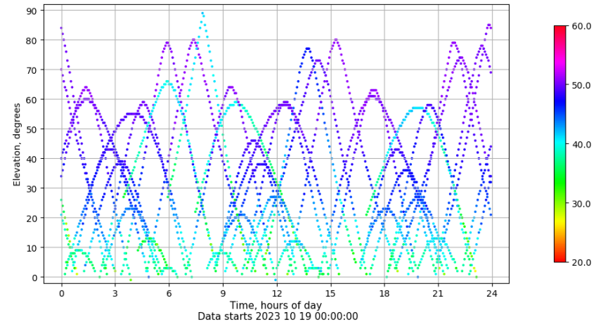
Time-elevation plot for station IBIZ. Signal to Noise S1C Data file IBIZ00ESP_R_2023292.xtr
