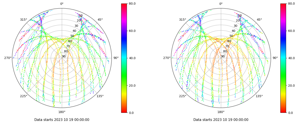
Skyplot for station IBIZ. Parameter M1C Data file IBIZ00ESP_R_2023292.xtr Skyplot for station IBIZ. Parameter M2P Data file IBIZ00ESP_R_2023292.xtr
