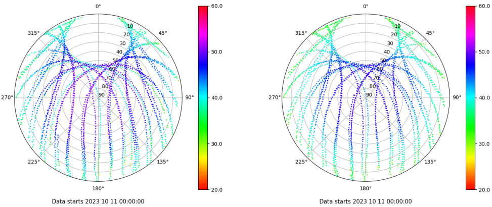
Skyplot for station IBIZ. Signal to Noise S1C Data file IBIZ00ESP_R_2023284.xtr Skyplot for station IBIZ. Signal to Noise S2P Data file IBIZ00ESP_R_2023284.xtr
