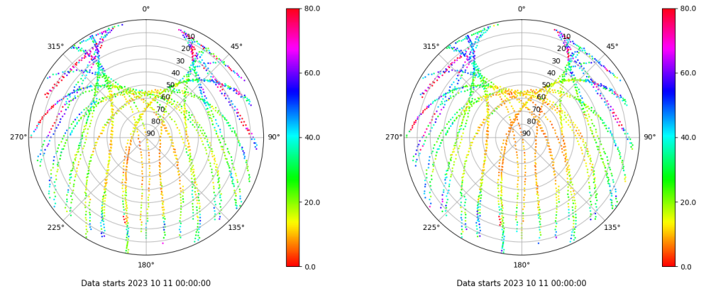
Skyplot for station IBIZ. Parameter M1C Data file IBIZ00ESP_R_2023284.xtr Skyplot for station IBIZ. Parameter M2P Data file IBIZ00ESP_R_2023284.xtr
