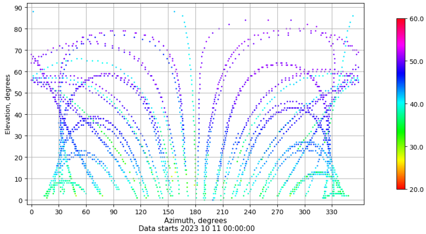
Azimuth-elevation plot for station IBIZ. Signal to Noise S1C Data file IBIZ00ESP_R_2023284.xtr
