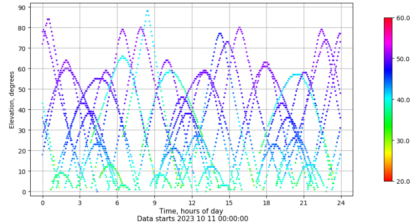
Time-elevation plot for station IBIZ. Signal to Noise S1C Data file IBIZ00ESP_R_2023284.xtr
