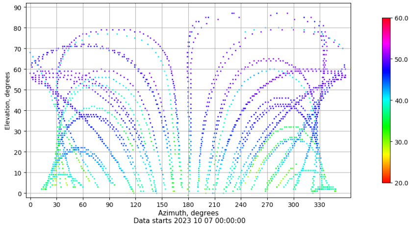
Azimuth-elevation plot for station IBIZ. Signal to Noise S1C Data file IBIZ00ESP_R_2023280.xtr
