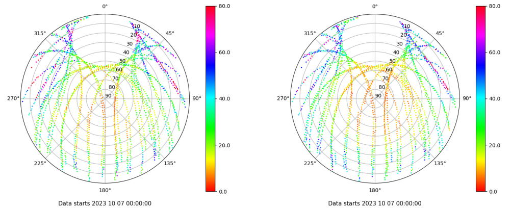
Skyplot for station IBIZ. Parameter M1C Data file IBIZ00ESP_R_2023280.xtr Skyplot for station IBIZ. Parameter M2P Data file IBIZ00ESP_R_2023280.xtr
