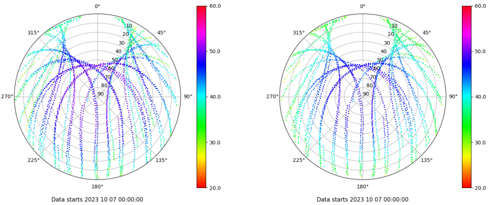
Skyplot for station IBIZ. Signal to Noise S1C Data file IBIZ00ESP_R_2023280.xtr Skyplot for station IBIZ. Signal to Noise S2P Data file IBIZ00ESP_R_2023280.xtr
