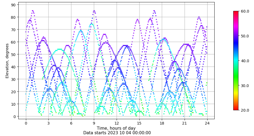
Time-elevation plot for station IBIZ. Signal to Noise S1C Data file IBIZ00ESP_R_2023277.xtr
