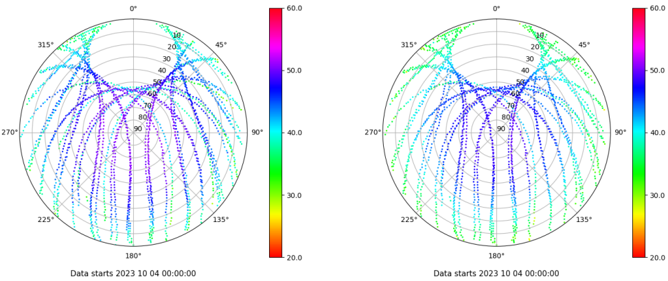
Skyplot for station IBIZ. Signal to Noise S1C Data file IBIZ00ESP_R_2023277.xtr Skyplot for station IBIZ. Signal to Noise S2P Data file IBIZ00ESP_R_2023277.xtr
