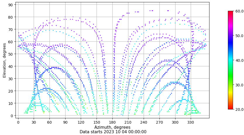
Azimuth-elevation plot for station IBIZ. Signal to Noise S1C Data file IBIZ00ESP_R_2023277.xtr
