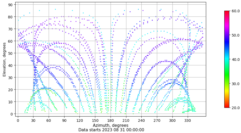
Azimuth-elevation plot for station IBIZ. Signal to Noise S1C Data file IBIZ00ESP_R_2023243.xtr
