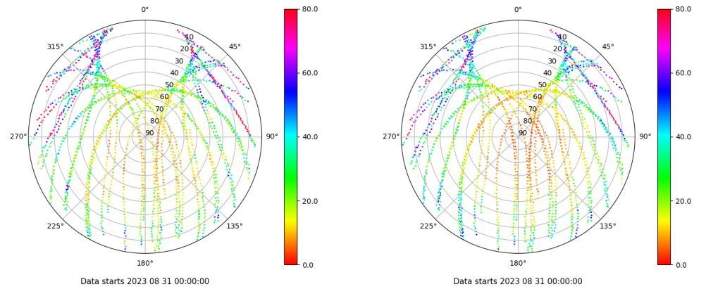
Skyplot for station IBIZ. Parameter M1C Data file IBIZ00ESP_R_2023243.xtr Skyplot for station IBIZ. Parameter M2P Data file IBIZ00ESP_R_2023243.xtr
