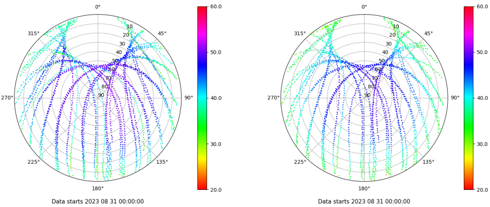
Skyplot for station IBIZ. Signal to Noise S1C Data file IBIZ00ESP_R_2023243.xtr Skyplot for station IBIZ. Signal to Noise S2P Data file IBIZ00ESP_R_2023243.xtr
