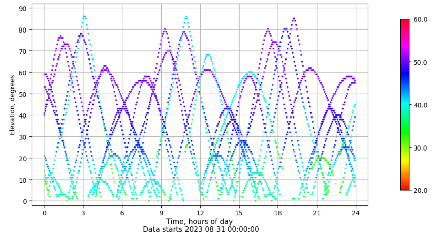
Time-elevation plot for station IBIZ. Signal to Noise S1C Data file IBIZ00ESP_R_2023243.xtr
