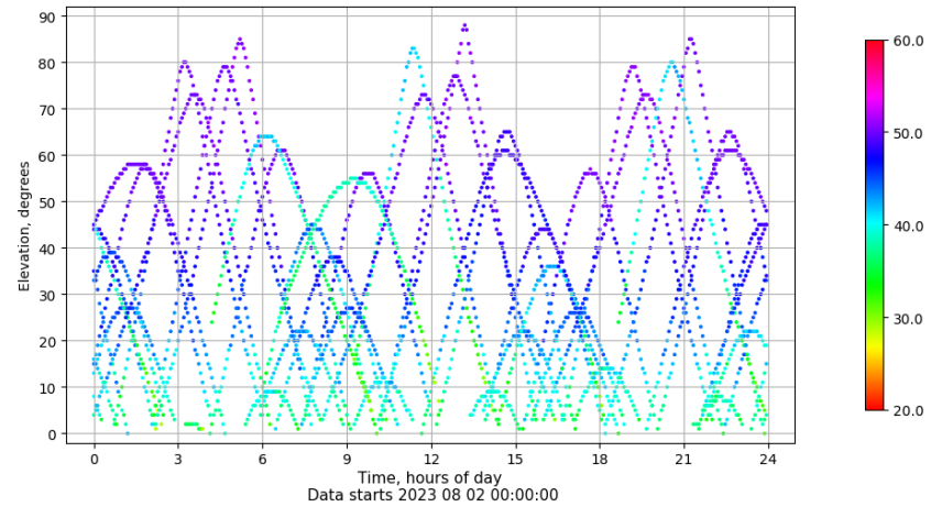
Time-elevation plot for station IBIZ. Signal to Noise S1C Data file IBIZ00ESP_R_2023214.xtr
