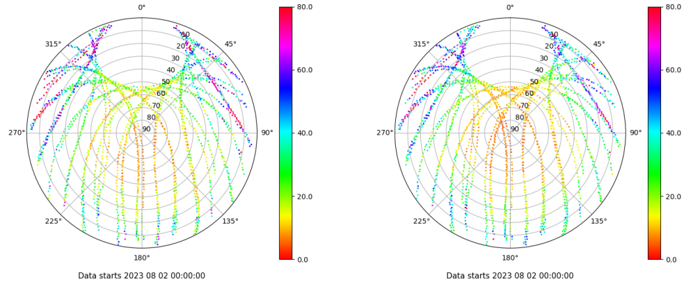
Skyplot for station IBIZ. Parameter M1C Data file IBIZ00ESP_R_2023214.xtr Skyplot for station IBIZ. Parameter M2P Data file IBIZ00ESP_R_2023214.xtr
