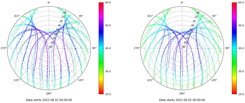
Skyplot for station IBIZ. Signal to Noise S1C Data file IBIZ00ESP_R_2023214.xtr Skyplot for station IBIZ. Signal to Noise S2P Data file IBIZ00ESP_R_2023214.xtr
