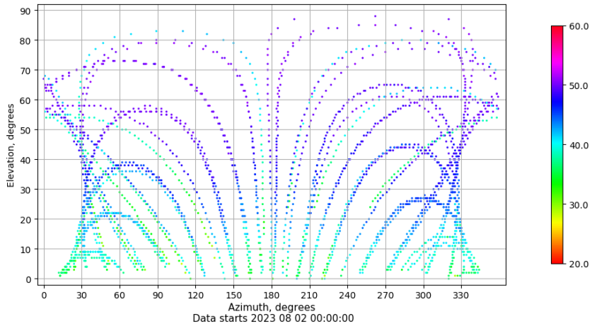
Azimuth-elevation plot for station IBIZ. Signal to Noise S1C Data file IBIZ00ESP_R_2023214.xtr
