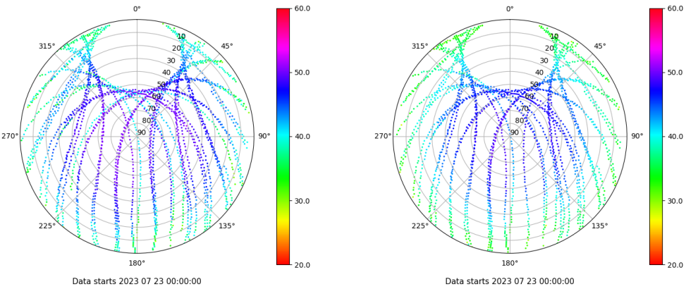
Skyplot for station IBIZ. Signal to Noise S1C Data file IBIZ00ESP_R_2023204.xtr Skyplot for station IBIZ. Signal to Noise S2P Data file IBIZ00ESP_R_2023204.xtr
