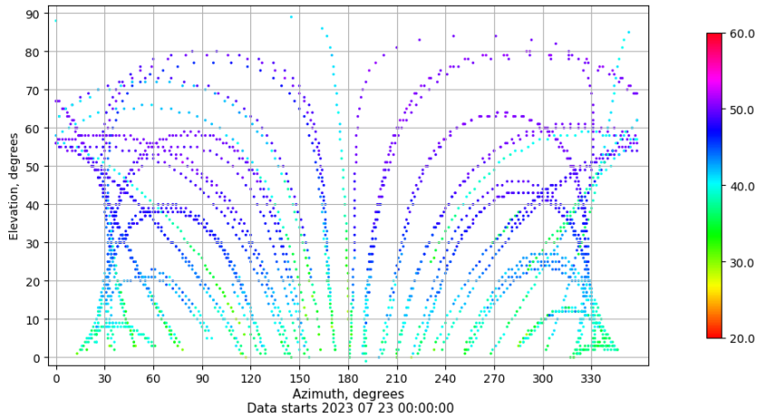
Azimuth-elevation plot for station IBIZ. Signal to Noise S1C Data file IBIZ00ESP_R_2023204.xtr
