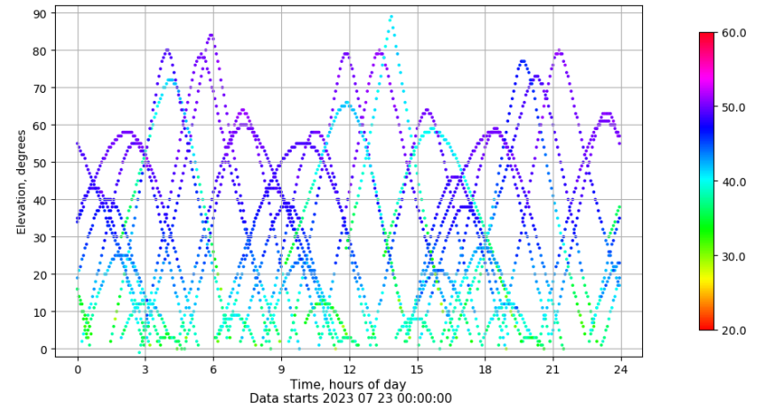
Time-elevation plot for station IBIZ. Signal to Noise S1C Data file IBIZ00ESP_R_2023204.xtr
