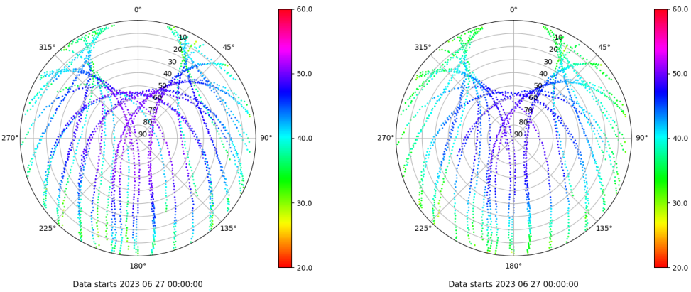
Skyplot for station IBIZ. Signal to Noise S1C Data file IBIZ00ESP_R_2023178.xtr Skyplot for station IBIZ. Signal to Noise S2P Data file IBIZ00ESP_R_2023178.xtr
