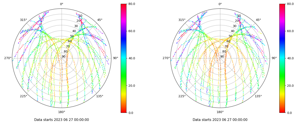
Skyplot for station IBIZ. Parameter M1C Data file IBIZ00ESP_R_2023178.xtr Skyplot for station IBIZ. Parameter M2P Data file IBIZ00ESP_R_2023178.xtr
