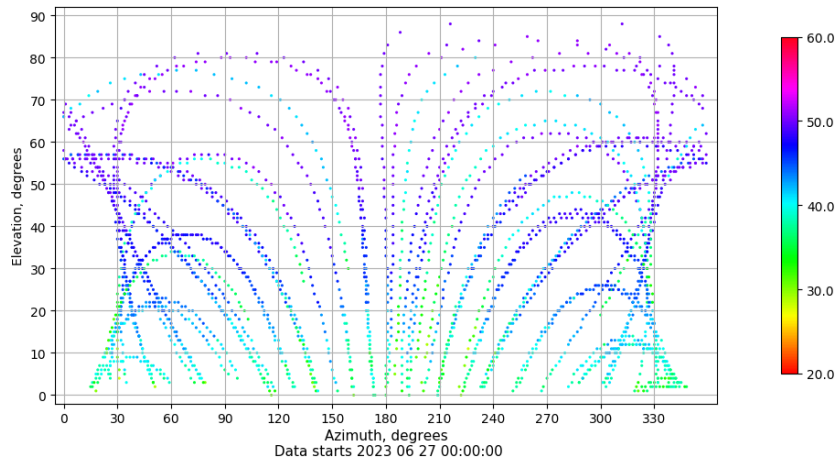
Azimuth-elevation plot for station IBIZ. Signal to Noise S1C Data file IBIZ00ESP_R_2023178.xtr
