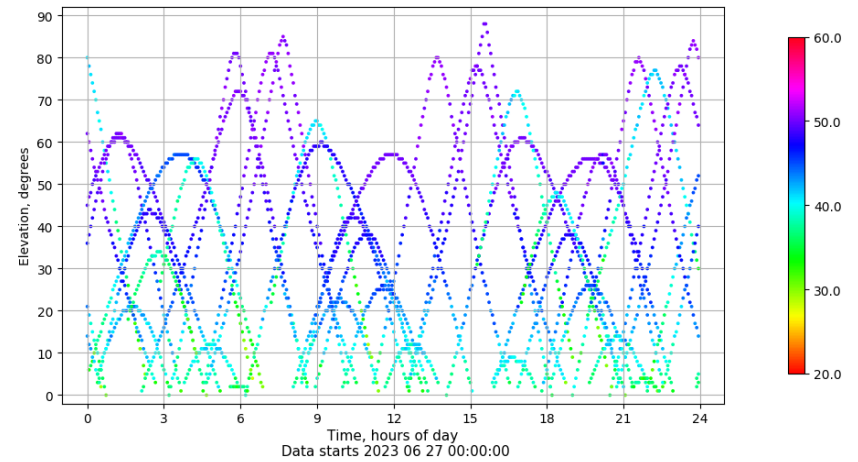
Time-elevation plot for station IBIZ. Signal to Noise S1C Data file IBIZ00ESP_R_2023178.xtr
