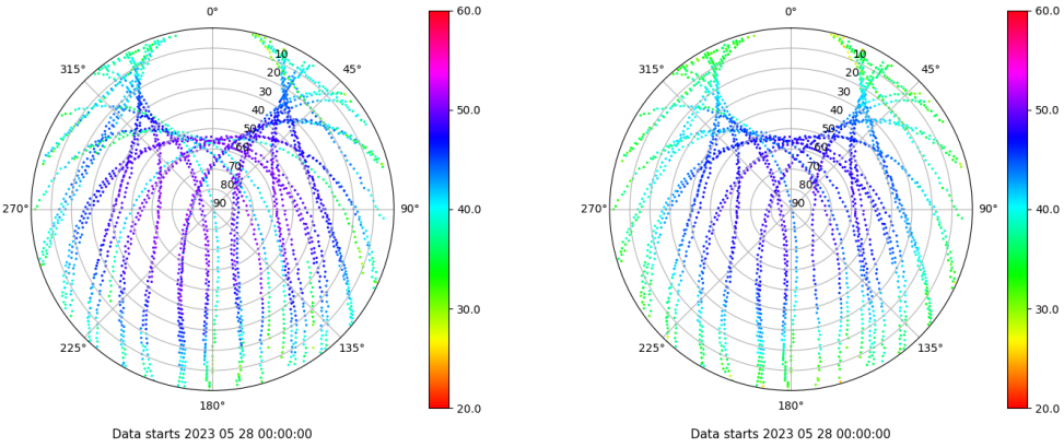
Skyplot for station IBIZ. Signal to Noise S1C Data file IBIZ00ESP_R_2023148.xtr Skyplot for station IBIZ. Signal to Noise S2P Data file IBIZ00ESP_R_2023148.xtr
