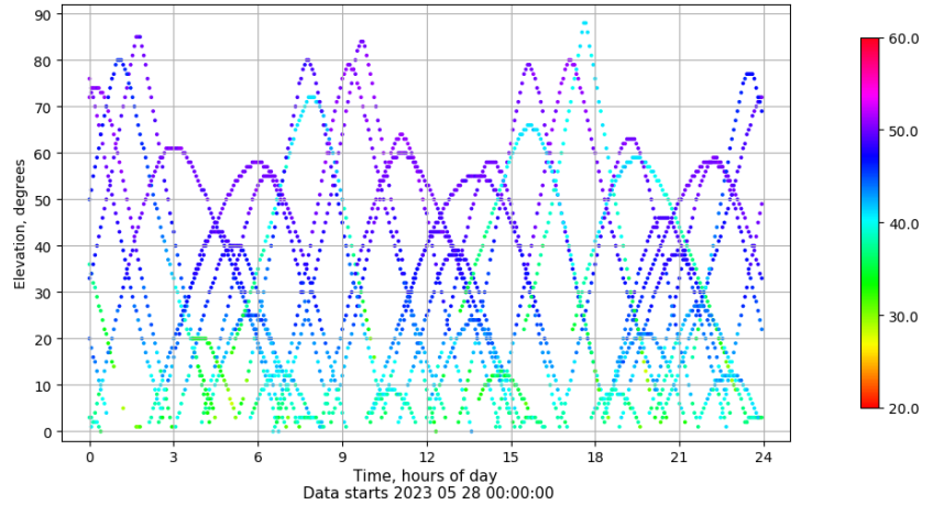
Time-elevation plot for station IBIZ. Signal to Noise S1C Data file IBIZ00ESP_R_2023148.xtr
