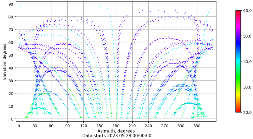
Azimuth-elevation plot for station IBIZ. Signal to Noise S1C Data file IBIZ00ESP_R_2023148.xtr
