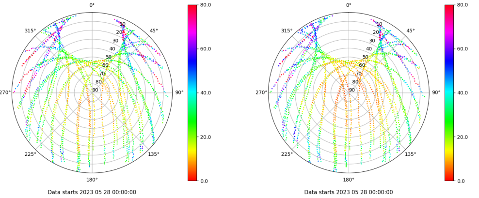
Skyplot for station IBIZ. Parameter M1C Data file IBIZ00ESP_R_2023148.xtr Skyplot for station IBIZ. Parameter M2P Data file IBIZ00ESP_R_2023148.xtr
