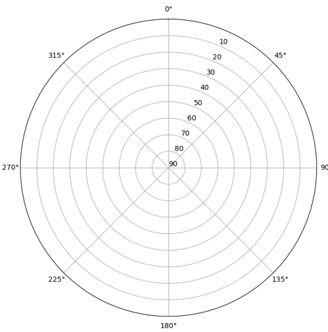
Skyplot for station IBIZ. Parameter M1C Data file IBIZ00ESP_R_2023129.xtr
