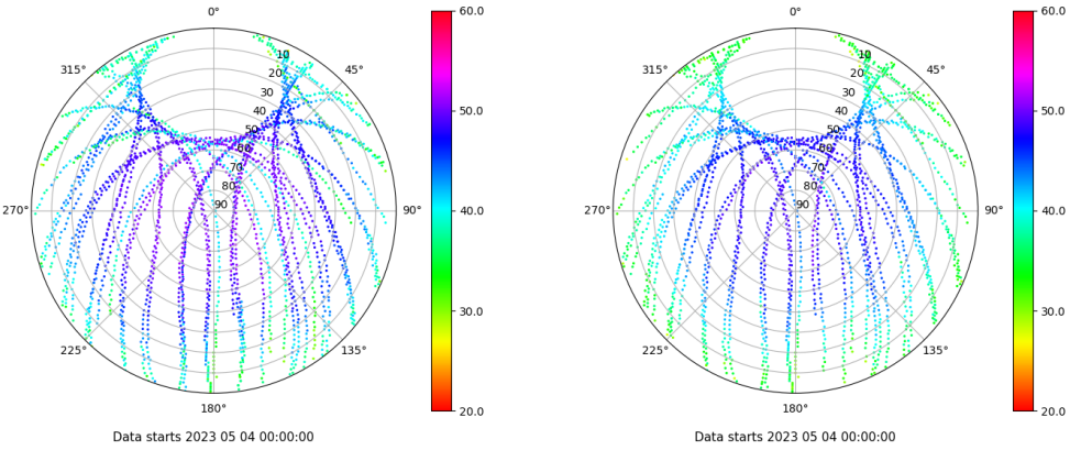
Skyplot for station IBIZ. Signal to Noise S1C Data file IBIZ00ESP_R_2023124.xtr Skyplot for station IBIZ. Signal to Noise S2P Data file IBIZ00ESP_R_2023124.xtr
