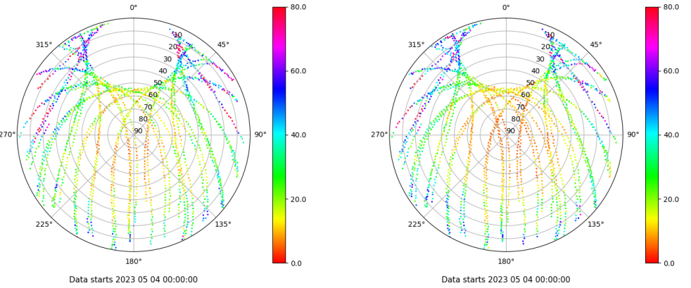
Skyplot for station IBIZ. Parameter M1C Data file IBIZ00ESP_R_2023124.xtr Skyplot for station IBIZ. Parameter M2P Data file IBIZ00ESP_R_2023124.xtr
