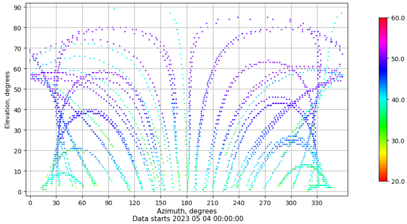
Azimuth-elevation plot for station IBIZ. Signal to Noise S1C Data file IBIZ00ESP_R_2023124.xtr
