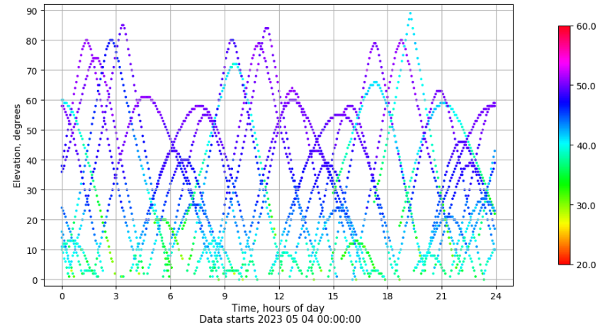
Time-elevation plot for station IBIZ. Signal to Noise S1C Data file IBIZ00ESP_R_2023124.xtr
