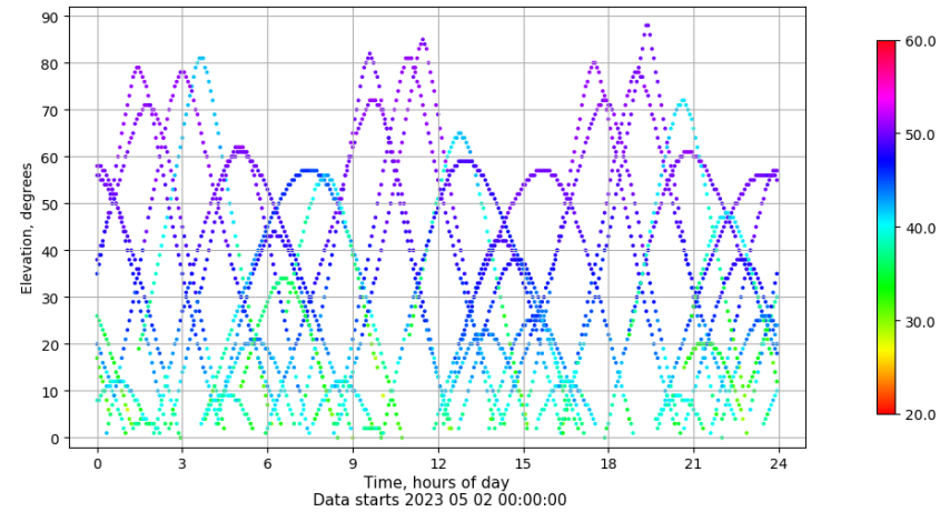
Time-elevation plot for station IBIZ. Signal to Noise S1C Data file IBIZ00ESP_R_2023122.xtr
