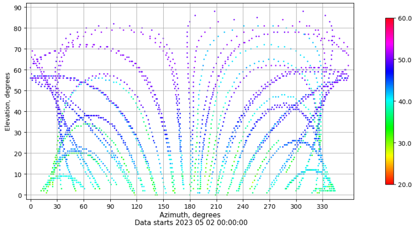
Azimuth-elevation plot for station IBIZ. Signal to Noise S1C Data file IBIZ00ESP_R_2023122.xtr
