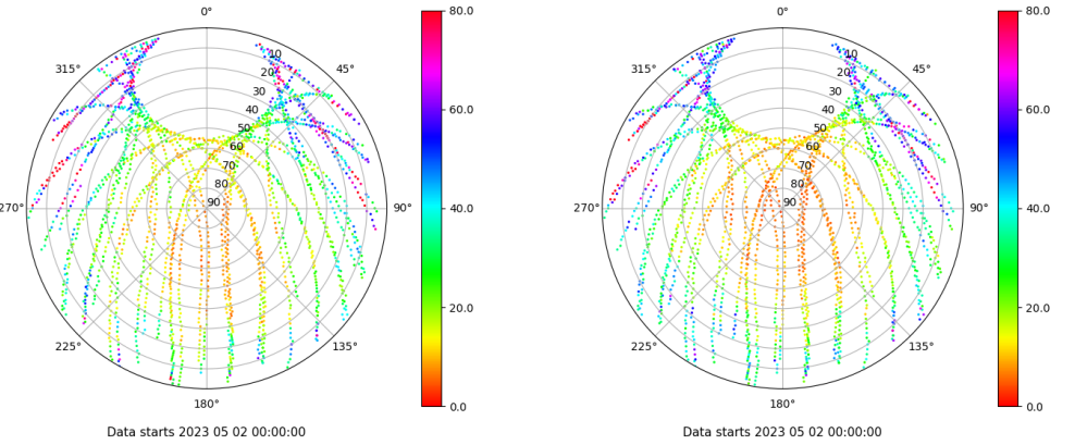
Skyplot for station IBIZ. Parameter M1C Data file IBIZ00ESP_R_2023122.xtr Skyplot for station IBIZ. Parameter M2P Data file IBIZ00ESP_R_2023122.xtr
