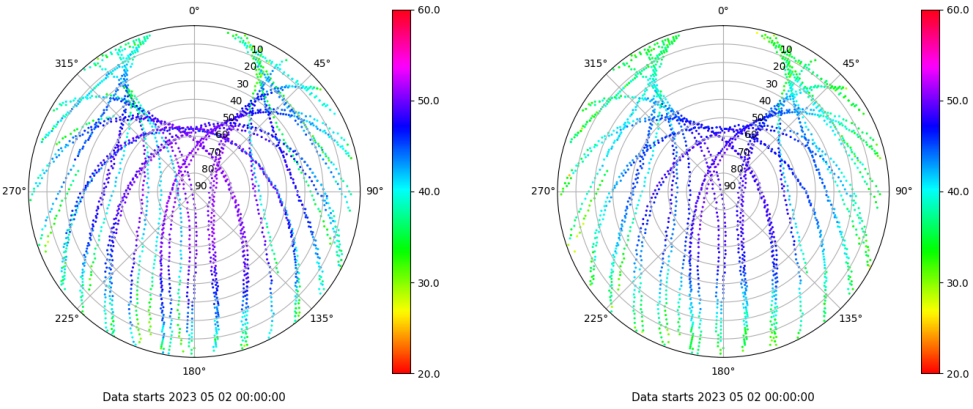
Skyplot for station IBIZ. Signal to Noise S1C Data file IBIZ00ESP_R_2023122.xtr Skyplot for station IBIZ. Signal to Noise S2P Data file IBIZ00ESP_R_2023122.xtr
