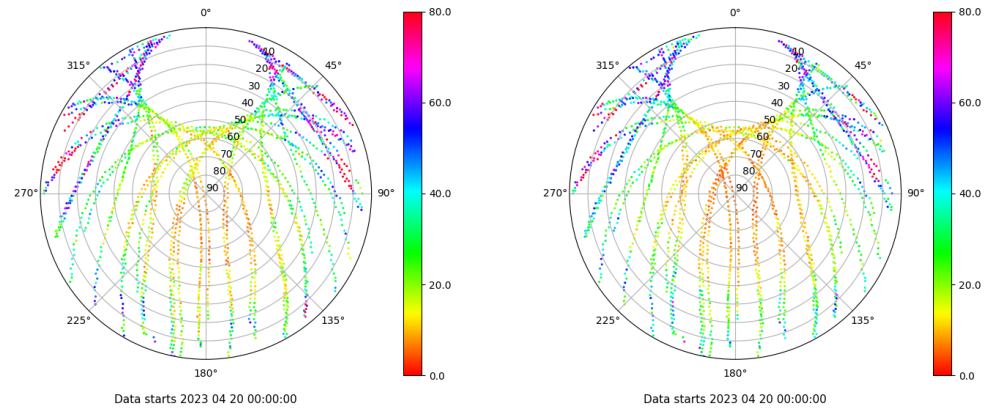
Skyplot for station IBIZ. Parameter M1C Data file IBIZ00ESP_R_2023110.xtr Skyplot for station IBIZ. Parameter M2P Data file IBIZ00ESP_R_2023110.xtr
