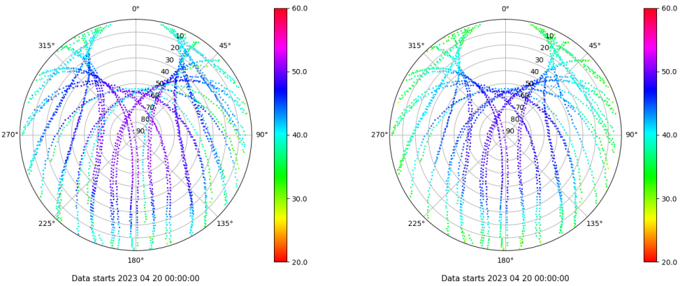
Skyplot for station IBIZ. Signal to Noise S1C Data file IBIZ00ESP_R_2023110.xtr Skyplot for station IBIZ. Signal to Noise S2P Data file IBIZ00ESP_R_2023110.xtr
