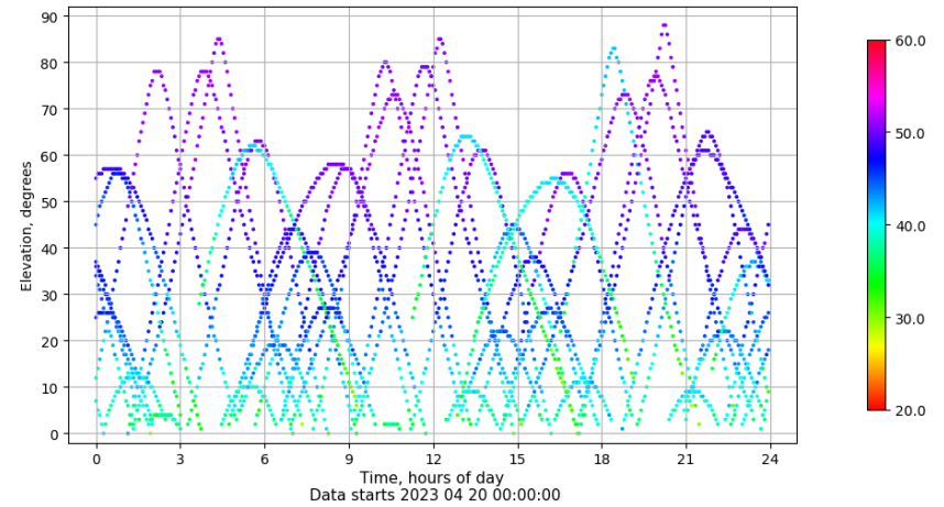
Time-elevation plot for station IBIZ. Signal to Noise S1C Data file IBIZ00ESP_R_2023110.xtr
