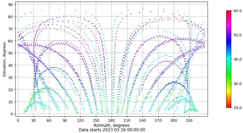
Azimuth-elevation plot for station IBIZ. Signal to Noise S1C Data file IBIZ00ESP_R_2023075.xtr
