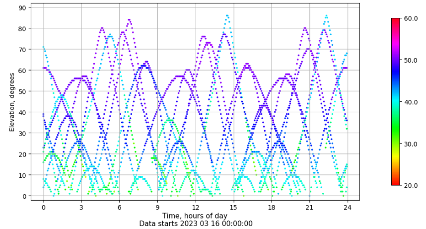
Time-elevation plot for station IBIZ. Signal to Noise S1C Data file IBIZ00ESP_R_2023075.xtr
