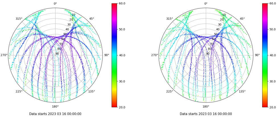
Skyplot for station IBIZ. Signal to Noise S1C Data file IBIZ00ESP_R_2023075.xtr Skyplot for station IBIZ. Signal to Noise S2P Data file IBIZ00ESP_R_2023075.xtr
