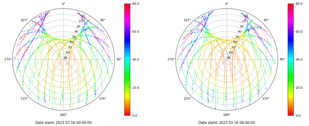
Skyplot for station IBIZ. Parameter M1C Data file IBIZ00ESP_R_2023075.xtr Skyplot for station IBIZ. Parameter M2P Data file IBIZ00ESP_R_2023075.xtr
