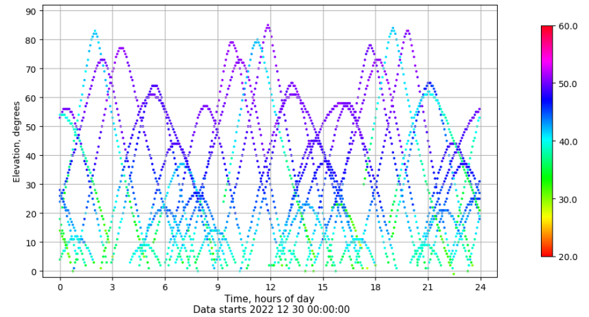
Time-elevation plot for station IBIZ. Signal to Noise S1C Data file IBIZ00ESP_R_2022364.xtr
