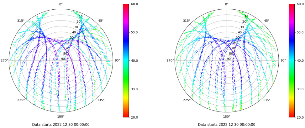
Skyplot for station IBIZ. Signal to Noise S1C Data file IBIZ00ESP_R_2022364.xtr Skyplot for station IBIZ. Signal to Noise S2P Data file IBIZ00ESP_R_2022364.xtr
