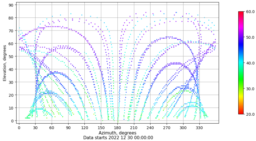
Azimuth-elevation plot for station IBIZ. Signal to Noise S1C Data file IBIZ00ESP_R_2022364.xtr
