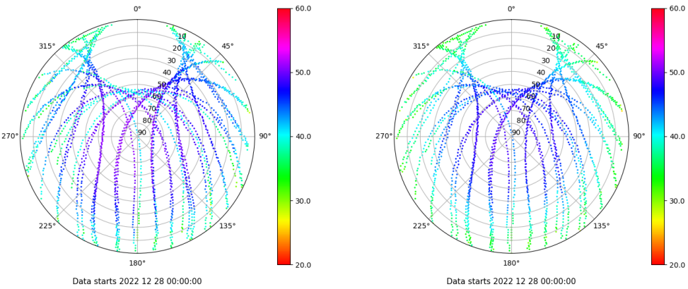
Skyplot for station IBIZ. Signal to Noise S1C Data file IBIZ00ESP_R_2022362.xtr Skyplot for station IBIZ. Signal to Noise S2P Data file IBIZ00ESP_R_2022362.xtr
