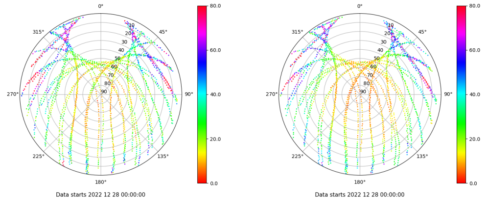
Skyplot for station IBIZ. Parameter M1C Data file IBIZ00ESP_R_2022362.xtr Skyplot for station IBIZ. Parameter M2P Data file IBIZ00ESP_R_2022362.xtr
