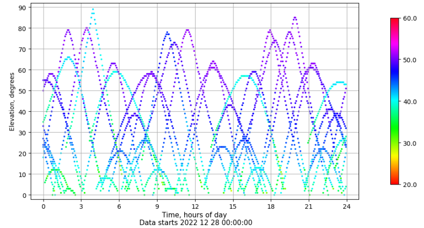
Time-elevation plot for station IBIZ. Signal to Noise S1C Data file IBIZ00ESP_R_2022362.xtr
