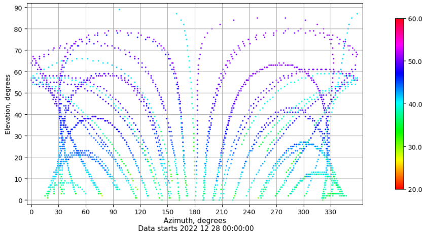
Azimuth-elevation plot for station IBIZ. Signal to Noise S1C Data file IBIZ00ESP_R_2022362.xtr
