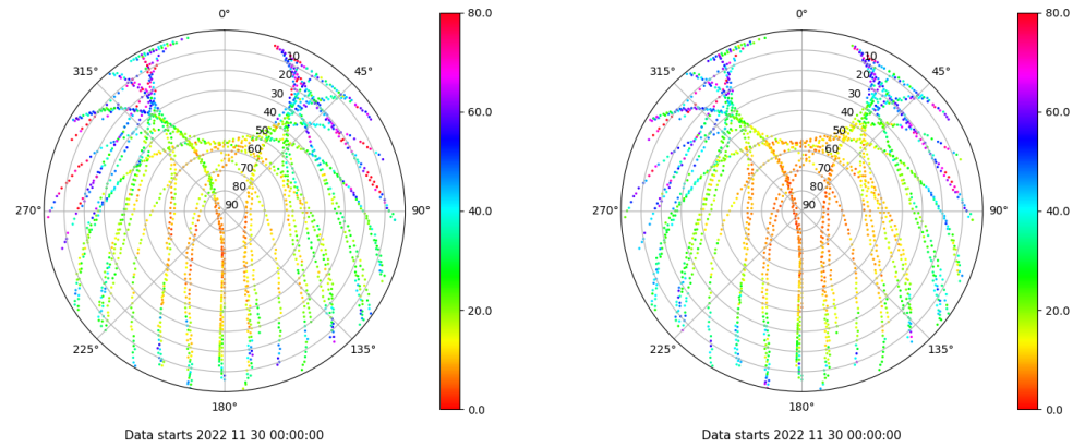
Skyplot for station IBIZ. Parameter M1C Data file IBIZ00ESP_R_2022334.xtr Skyplot for station IBIZ. Parameter M2P Data file IBIZ00ESP_R_2022334.xtr
