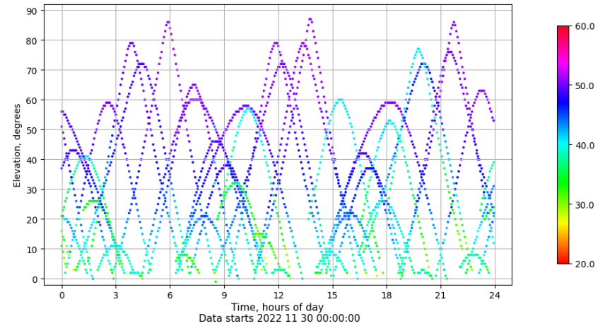
Time-elevation plot for station IBIZ. Signal to Noise S1C Data file IBIZ00ESP_R_2022334.xtr
