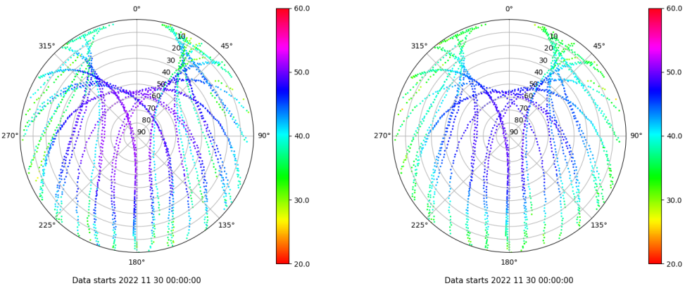
Skyplot for station IBIZ. Signal to Noise S1C Data file IBIZ00ESP_R_2022334.xtr Skyplot for station IBIZ. Signal to Noise S2P Data file IBIZ00ESP_R_2022334.xtr
