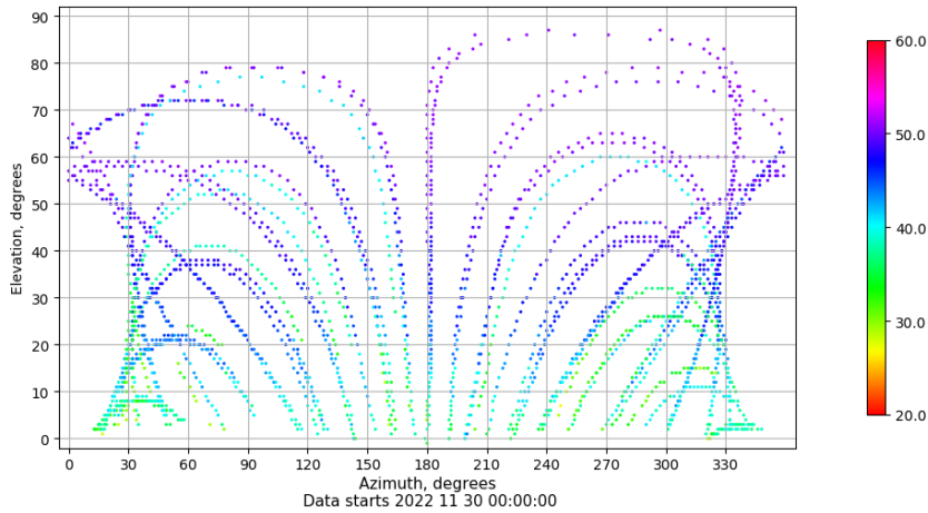
Azimuth-elevation plot for station IBIZ. Signal to Noise S1C Data file IBIZ00ESP_R_2022334.xtr
