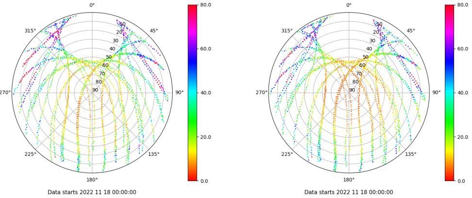
Skyplot for station IBIZ. Parameter M1C Data file IBIZ00ESP_R_2022322.xtr Skyplot for station IBIZ. Parameter M2P Data file IBIZ00ESP_R_2022322.xtr
