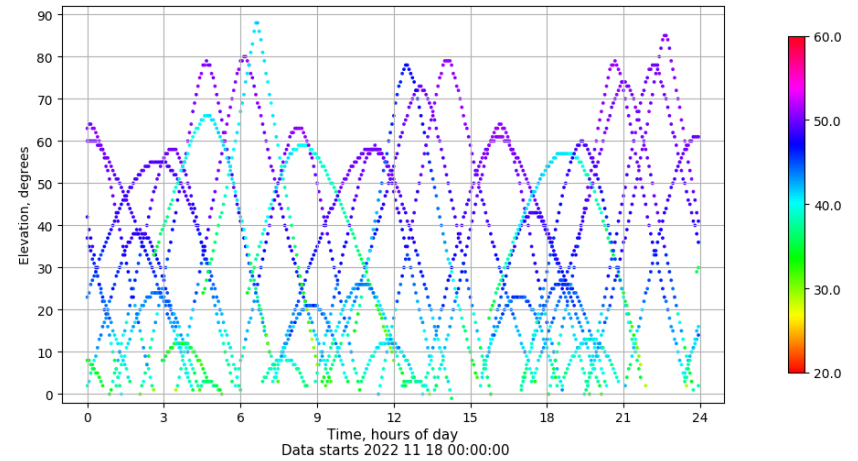
Time-elevation plot for station IBIZ. Signal to Noise S1C Data file IBIZ00ESP_R_2022322.xtr
