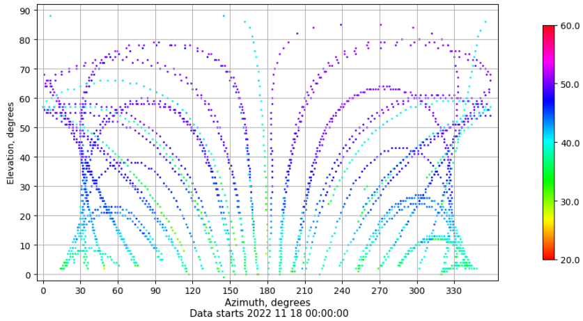
Azimuth-elevation plot for station IBIZ. Signal to Noise S1C Data file IBIZ00ESP_R_2022322.xtr
