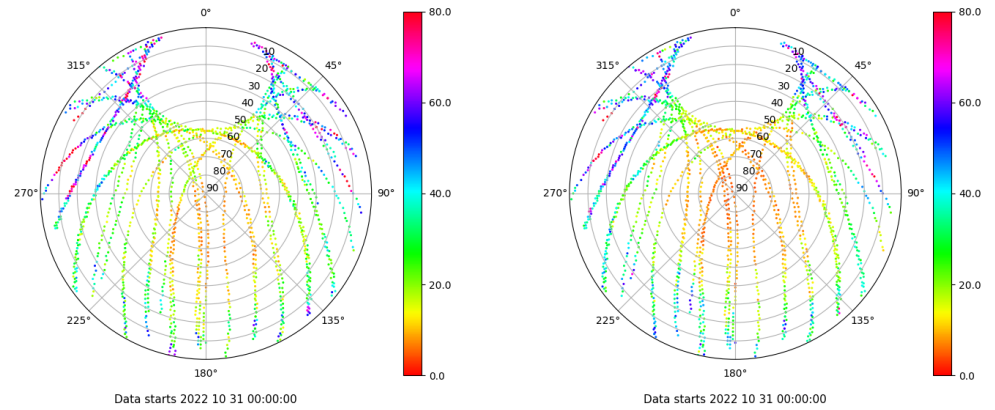
Skyplot for station IBIZ. Parameter M1C Data file IBIZ00ESP_R_2022304.xtr Skyplot for station IBIZ. Parameter M2P Data file IBIZ00ESP_R_2022304.xtr
