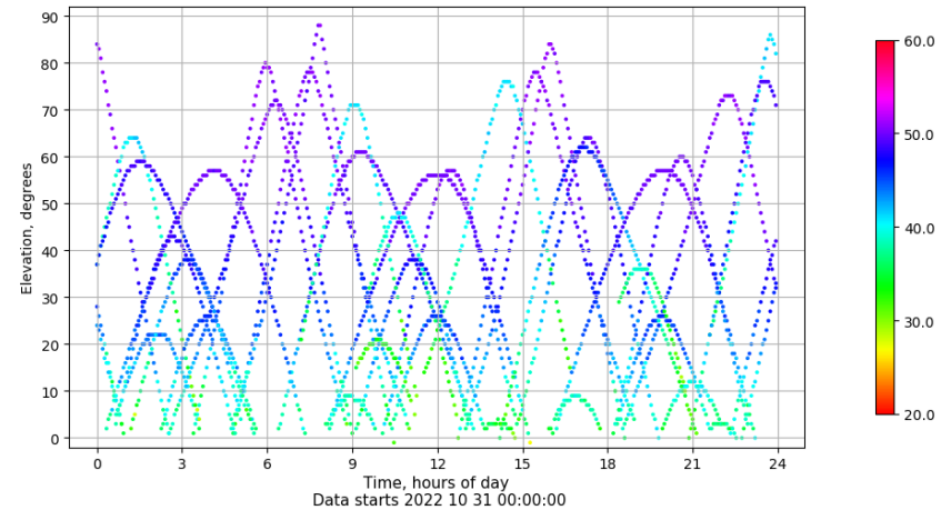
Time-elevation plot for station IBIZ. Signal to Noise S1C Data file IBIZ00ESP_R_2022304.xtr
