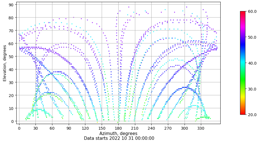
Azimuth-elevation plot for station IBIZ. Signal to Noise S1C Data file IBIZ00ESP_R_2022304.xtr
