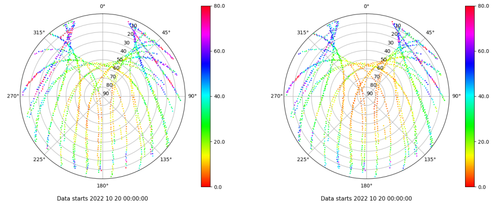
Skyplot for station IBIZ. Parameter M1C Data file IBIZ00ESP_R_2022293.xtr Skyplot for station IBIZ. Parameter M2P Data file IBIZ00ESP_R_2022293.xtr
