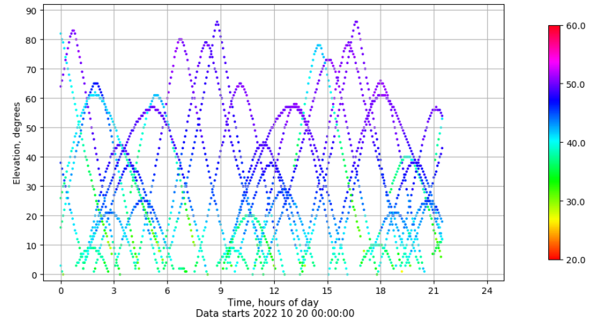
Time-elevation plot for station IBIZ. Signal to Noise S1C Data file IBIZ00ESP_R_2022293.xtr
