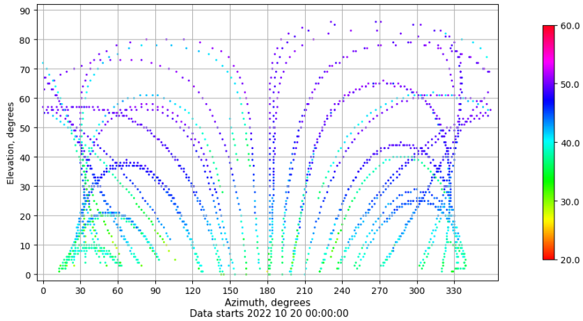
Azimuth-elevation plot for station IBIZ. Signal to Noise S1C Data file IBIZ00ESP_R_2022293.xtr
