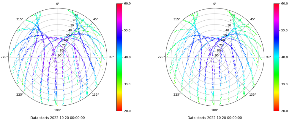
Skyplot for station IBIZ. Signal to Noise S1C Data file IBIZ00ESP_R_2022293.xtr Skyplot for station IBIZ. Signal to Noise S2P Data file IBIZ00ESP_R_2022293.xtr
