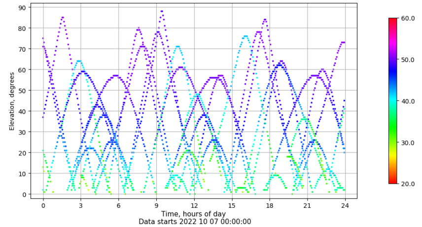
Time-elevation plot for station IBIZ. Signal to Noise S1C Data file IBIZ00ESP_R_2022280.xtr
