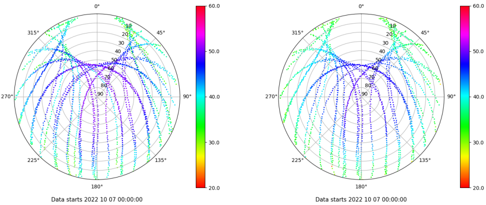
Skyplot for station IBIZ. Signal to Noise S1C Data file IBIZ00ESP_R_2022280.xtr Skyplot for station IBIZ. Signal to Noise S2P Data file IBIZ00ESP_R_2022280.xtr
