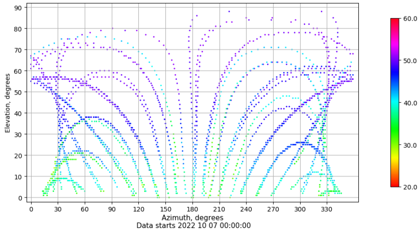
Azimuth-elevation plot for station IBIZ. Signal to Noise S1C Data file IBIZ00ESP_R_2022280.xtr
