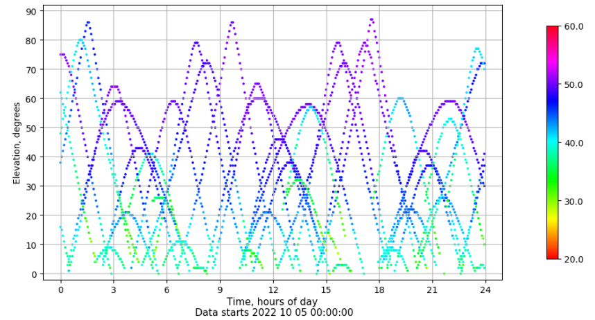
Time-elevation plot for station IBIZ. Signal to Noise S1C Data file IBIZ00ESP_R_2022278.xtr
