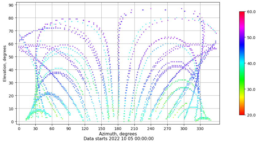
Azimuth-elevation plot for station IBIZ. Signal to Noise S1C Data file IBIZ00ESP_R_2022278.xtr
