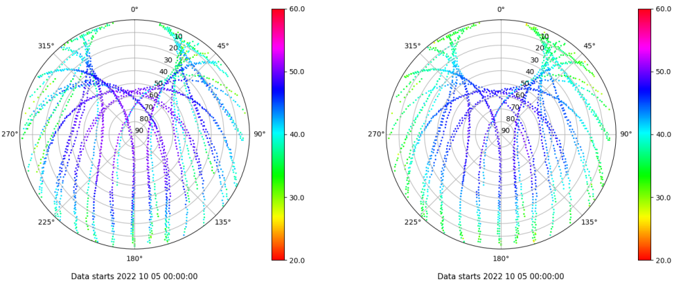
Skyplot for station IBIZ. Signal to Noise S1C Data file IBIZ00ESP_R_2022278.xtr Skyplot for station IBIZ. Signal to Noise S2P Data file IBIZ00ESP_R_2022278.xtr
