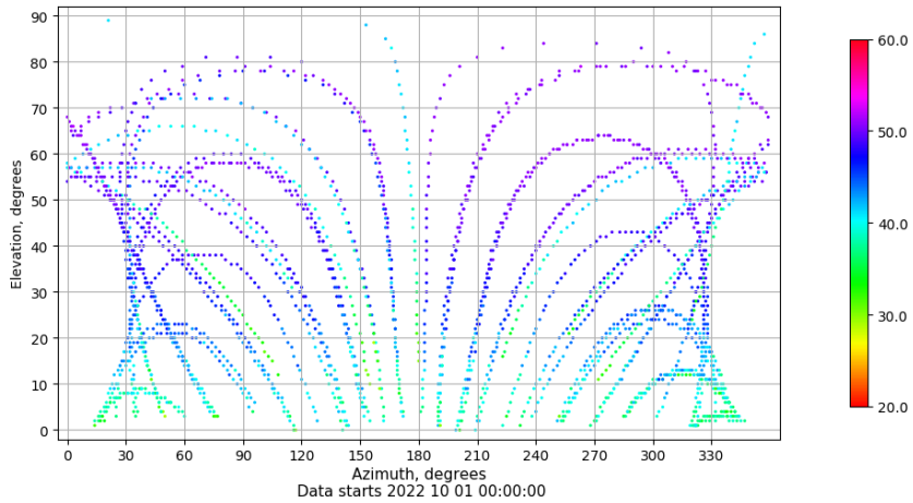
Azimuth-elevation plot for station IBIZ. Signal to Noise S1C Data file IBIZ00ESP_R_2022274.xtr
