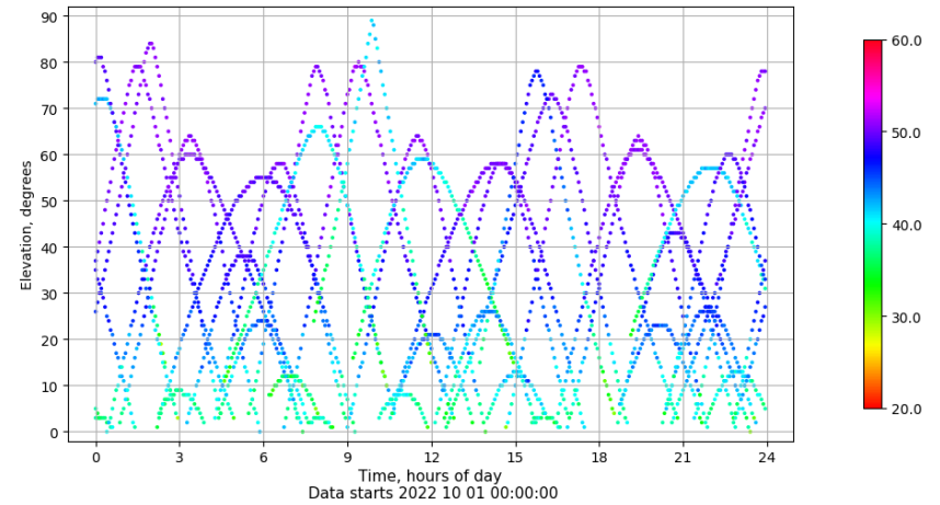
Time-elevation plot for station IBIZ. Signal to Noise S1C Data file IBIZ00ESP_R_2022274.xtr
