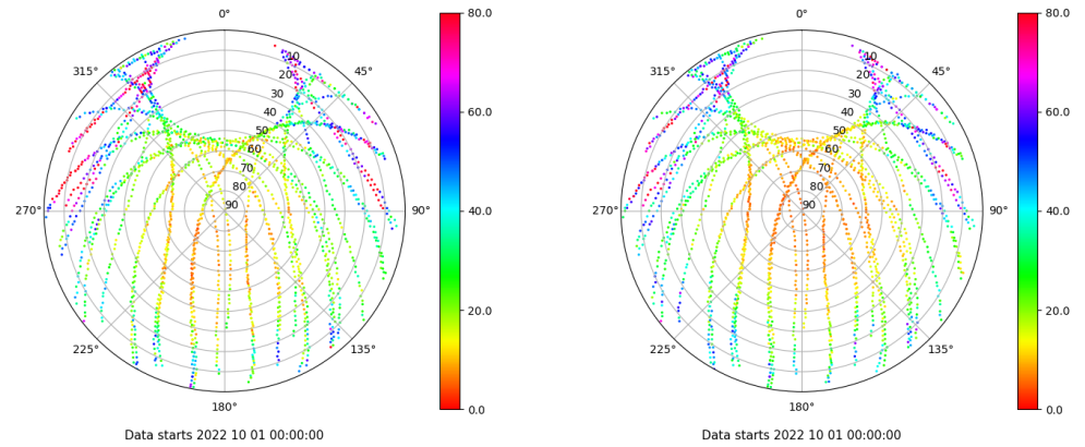
Skyplot for station IBIZ. Parameter M1C Data file IBIZ00ESP_R_2022274.xtr Skyplot for station IBIZ. Parameter M2P Data file IBIZ00ESP_R_2022274.xtr
