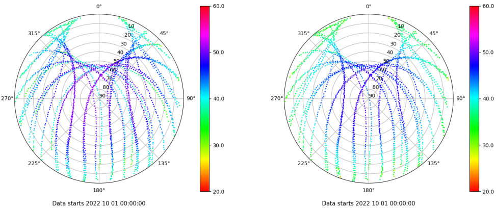
Skyplot for station IBIZ. Signal to Noise S1C Data file IBIZ00ESP_R_2022274.xtr Skyplot for station IBIZ. Signal to Noise S2P Data file IBIZ00ESP_R_2022274.xtr
