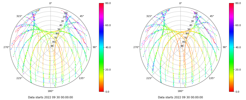
Skyplot for station IBIZ. Parameter M1C Data file IBIZ00ESP_R_2022273.xtr Skyplot for station IBIZ. Parameter M2P Data file IBIZ00ESP_R_2022273.xtr
