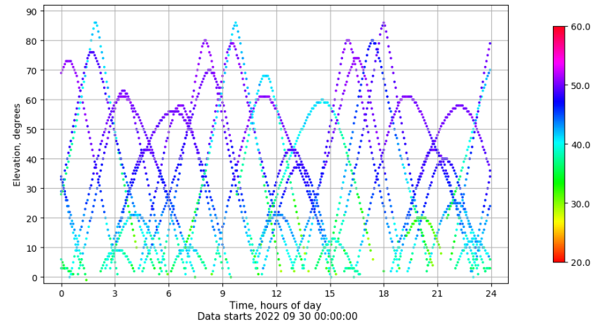
Time-elevation plot for station IBIZ. Signal to Noise S1C Data file IBIZ00ESP_R_2022273.xtr
