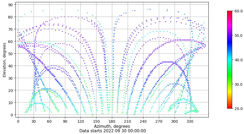
Azimuth-elevation plot for station IBIZ. Signal to Noise S1C Data file IBIZ00ESP_R_2022273.xtr
