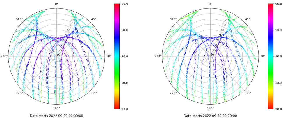
Skyplot for station IBIZ. Signal to Noise S1C Data file IBIZ00ESP_R_2022273.xtr Skyplot for station IBIZ. Signal to Noise S2P Data file IBIZ00ESP_R_2022273.xtr
