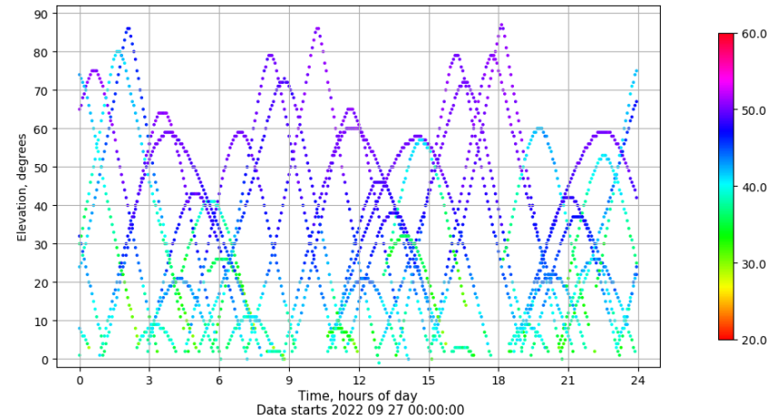
Time-elevation plot for station IBIZ. Signal to Noise S1C Data file IBIZ00ESP_R_2022270.xtr
