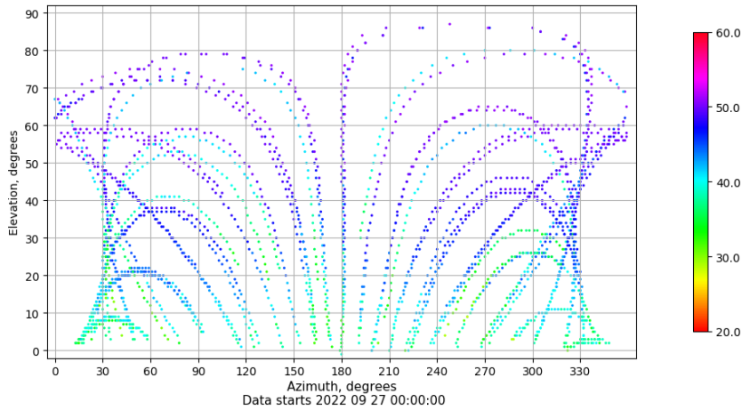
Azimuth-elevation plot for station IBIZ. Signal to Noise S1C Data file IBIZ00ESP_R_2022270.xtr
