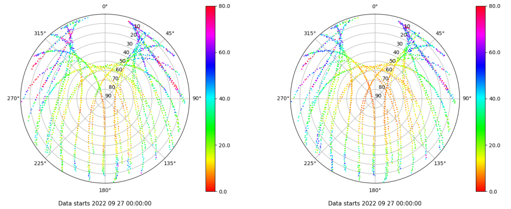
Skyplot for station IBIZ. Parameter M1C Data file IBIZ00ESP_R_2022270.xtr Skyplot for station IBIZ. Parameter M2P Data file IBIZ00ESP_R_2022270.xtr
