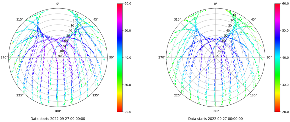
Skyplot for station IBIZ. Signal to Noise S1C Data file IBIZ00ESP_R_2022270.xtr Skyplot for station IBIZ. Signal to Noise S2P Data file IBIZ00ESP_R_2022270.xtr
