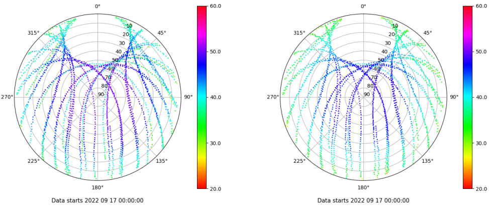
Skyplot for station IBIZ. Signal to Noise S1C Data file IBIZ00ESP_R_2022260.xtr Skyplot for station IBIZ. Signal to Noise S2P Data file IBIZ00ESP_R_2022260.xtr
