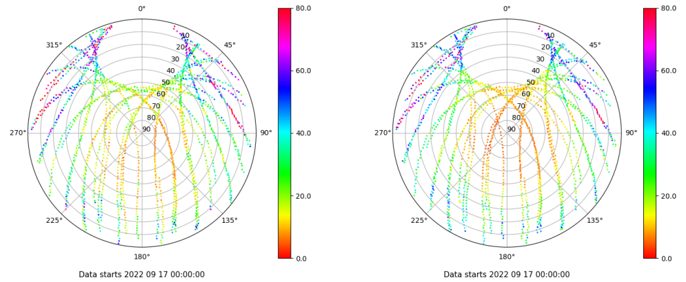
Skyplot for station IBIZ. Parameter M1C Data file IBIZ00ESP_R_2022260.xtr Skyplot for station IBIZ. Parameter M2P Data file IBIZ00ESP_R_2022260.xtr
