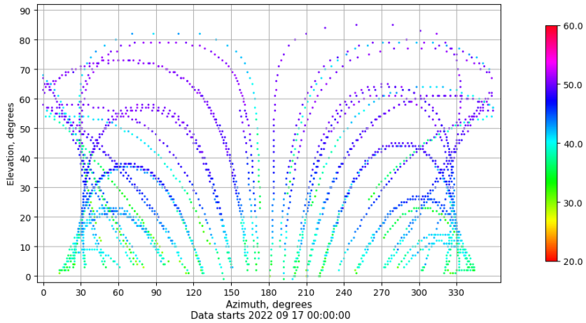
Azimuth-elevation plot for station IBIZ. Signal to Noise S1C Data file IBIZ00ESP_R_2022260.xtr
