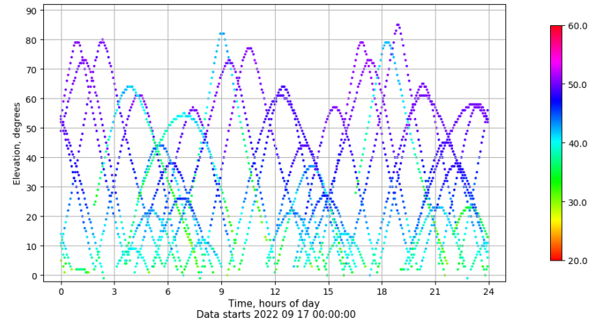
Time-elevation plot for station IBIZ. Signal to Noise S1C Data file IBIZ00ESP_R_2022260.xtr
