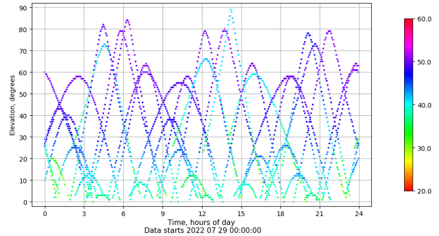
Time-elevation plot for station IBIZ. Signal to Noise S1C Data file IBIZ00ESP_R_2022210.xtr
