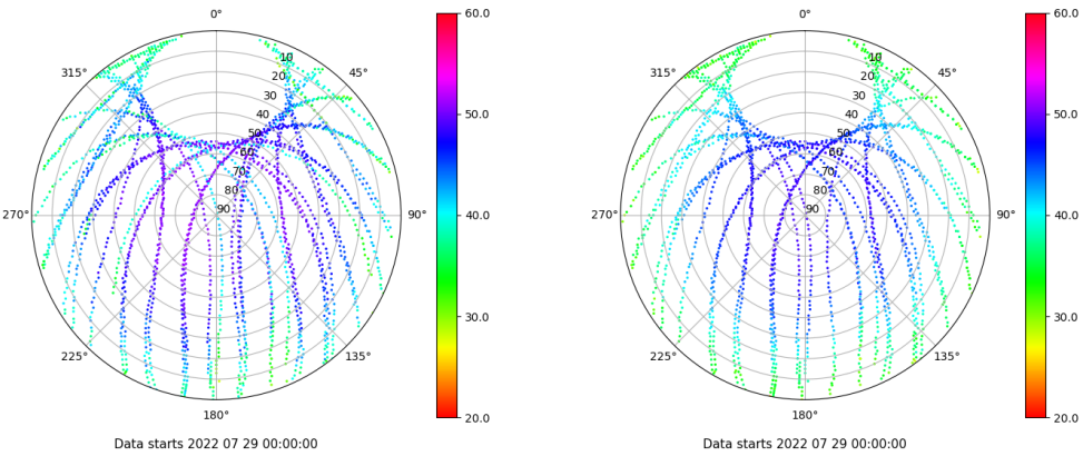
Skyplot for station IBIZ. Signal to Noise S1C Data file IBIZ00ESP_R_2022210.xtr Skyplot for station IBIZ. Signal to Noise S2P Data file IBIZ00ESP_R_2022210.xtr
