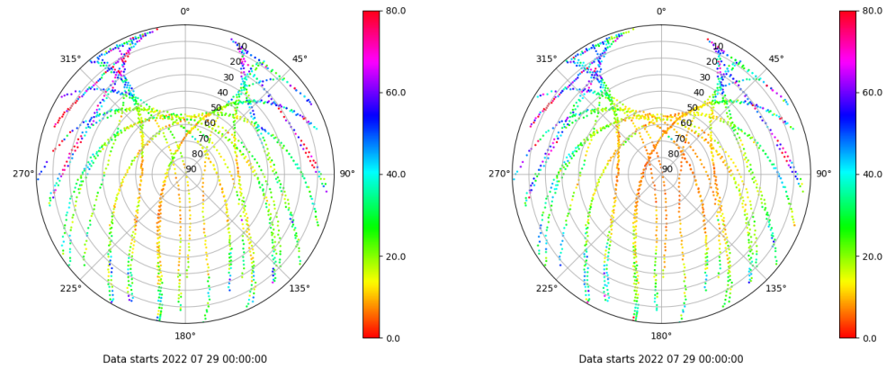
Skyplot for station IBIZ. Parameter M1C Data file IBIZ00ESP_R_2022210.xtr Skyplot for station IBIZ. Parameter M2P Data file IBIZ00ESP_R_2022210.xtr
