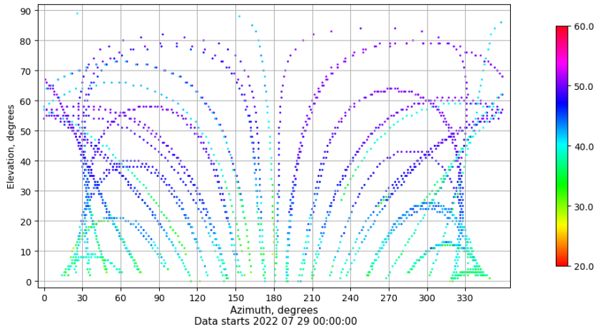
Azimuth-elevation plot for station IBIZ. Signal to Noise S1C Data file IBIZ00ESP_R_2022210.xtr
