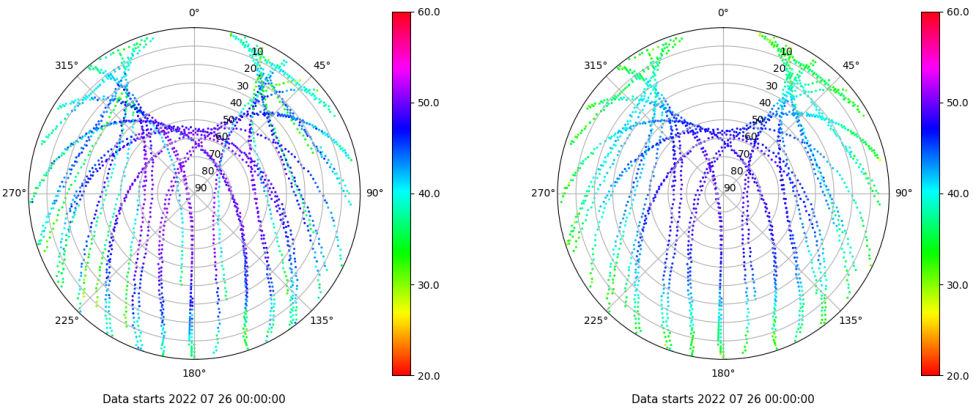
Skyplot for station IBIZ. Signal to Noise S1C Data file IBIZ00ESP_R_2022207.xtr Skyplot for station IBIZ. Signal to Noise S2P Data file IBIZ00ESP_R_2022207.xtr
