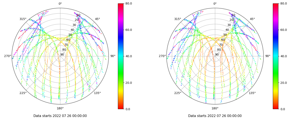
Skyplot for station IBIZ. Parameter M1C Data file IBIZ00ESP_R_2022207.xtr Skyplot for station IBIZ. Parameter M2P Data file IBIZ00ESP_R_2022207.xtr
