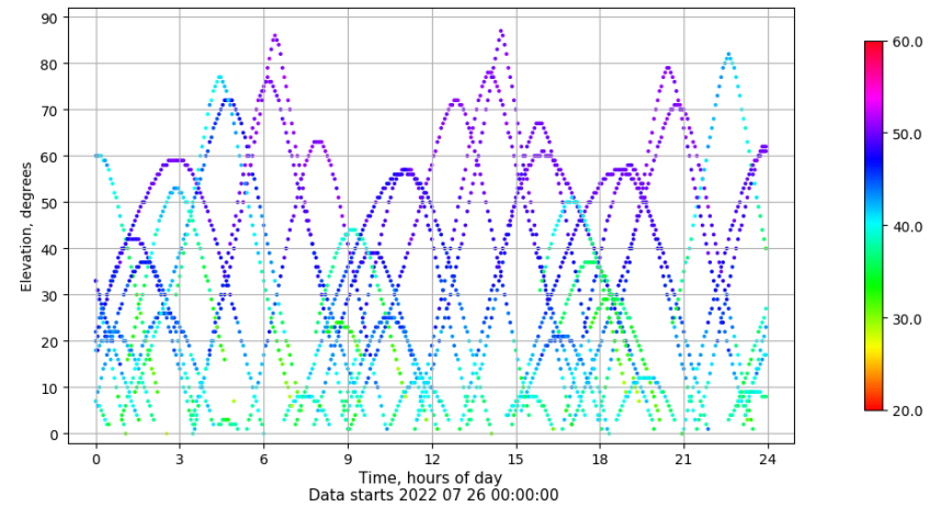
Time-elevation plot for station IBIZ. Signal to Noise S1C Data file IBIZ00ESP_R_2022207.xtr
