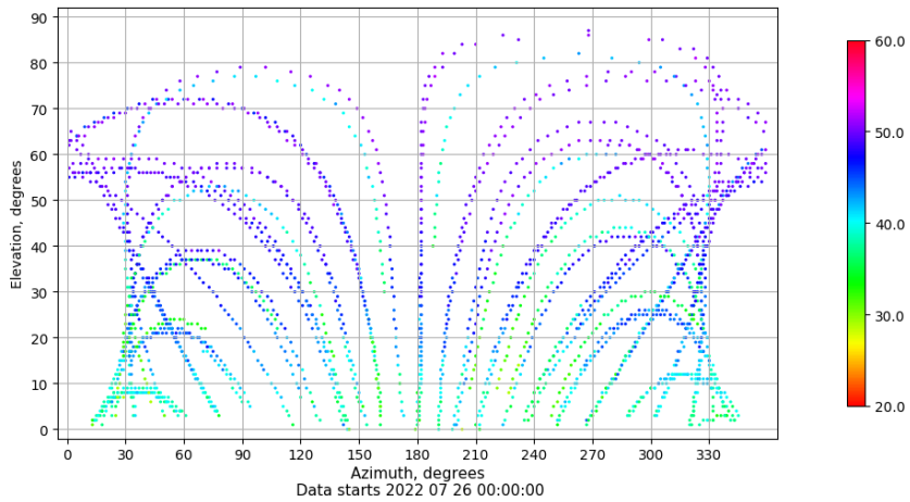
Azimuth-elevation plot for station IBIZ. Signal to Noise S1C Data file IBIZ00ESP_R_2022207.xtr
