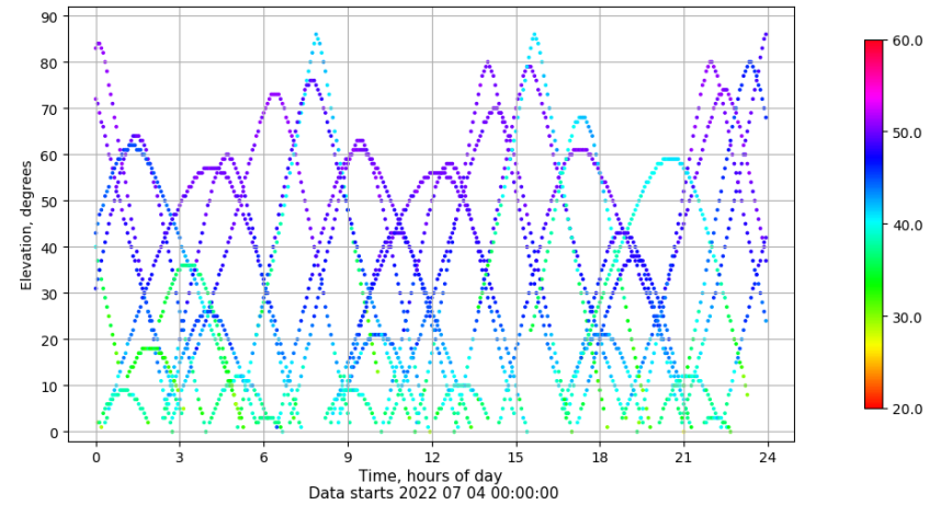
Time-elevation plot for station IBIZ. Signal to Noise S1C Data file IBIZ00ESP_R_2022185.xtr
