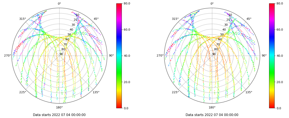
Skyplot for station IBIZ. Parameter M1C Data file IBIZ00ESP_R_2022185.xtr Skyplot for station IBIZ. Parameter M2P Data file IBIZ00ESP_R_2022185.xtr
