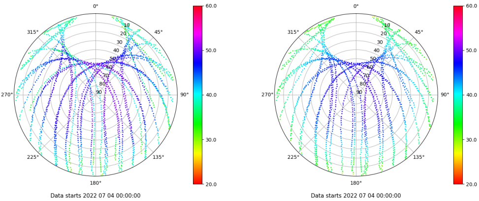
Skyplot for station IBIZ. Signal to Noise S1C Data file IBIZ00ESP_R_2022185.xtr Skyplot for station IBIZ. Signal to Noise S2P Data file IBIZ00ESP_R_2022185.xtr
