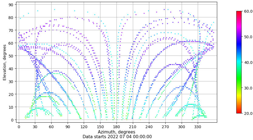
Azimuth-elevation plot for station IBIZ. Signal to Noise S1C Data file IBIZ00ESP_R_2022185.xtr
