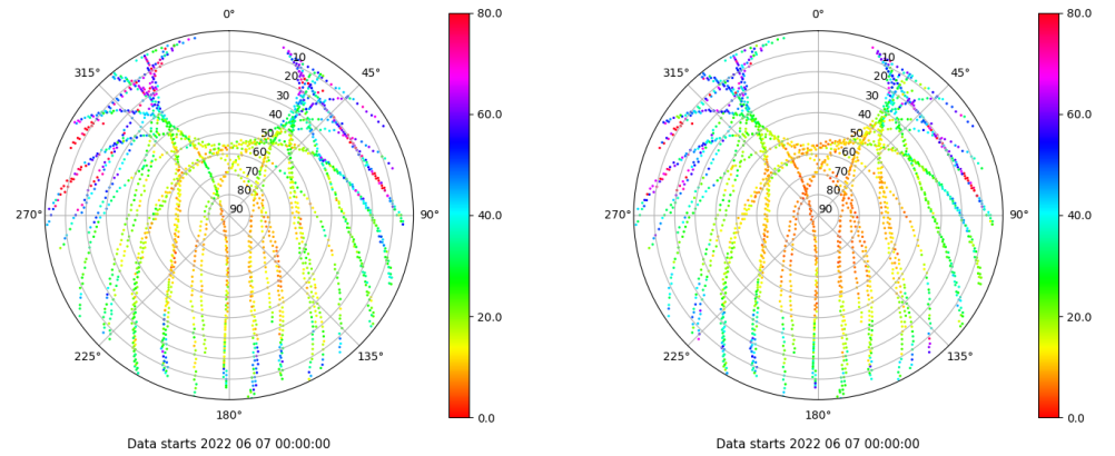
Skyplot for station IBIZ. Parameter M1C Data file IBIZ00ESP_R_2022158.xtr Skyplot for station IBIZ. Parameter M2P Data file IBIZ00ESP_R_2022158.xtr
