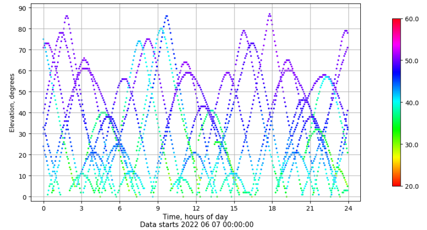
Time-elevation plot for station IBIZ. Signal to Noise S1C Data file IBIZ00ESP_R_2022158.xtr
