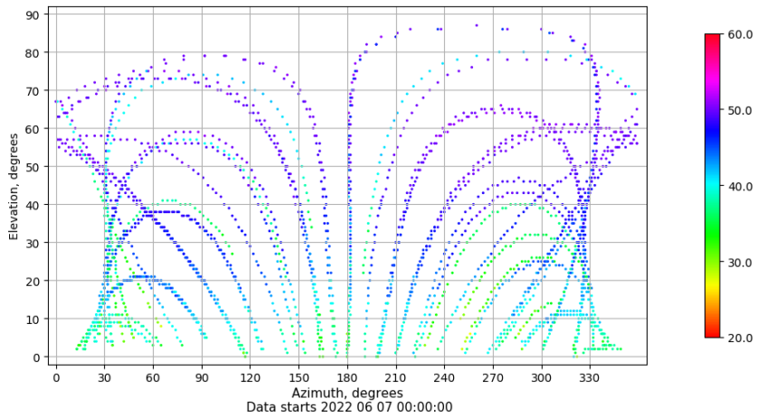
Azimuth-elevation plot for station IBIZ. Signal to Noise S1C Data file IBIZ00ESP_R_2022158.xtr
