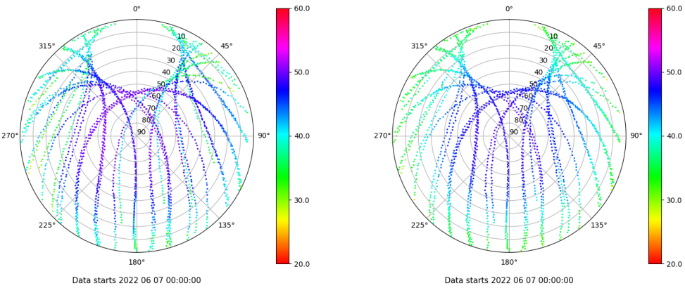
Skyplot for station IBIZ. Signal to Noise S1C Data file IBIZ00ESP_R_2022158.xtr Skyplot for station IBIZ. Signal to Noise S2P Data file IBIZ00ESP_R_2022158.xtr
