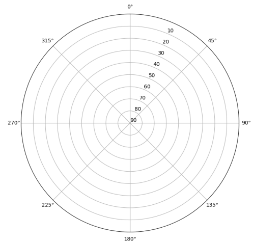
Skyplot for station IBIZ. Parameter M2P Data file IBIZ00ESP_R_2022050.xtr
