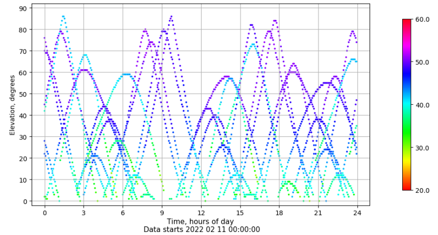
Time-elevation plot for station IBIZ. Signal to Noise S1C Data file IBIZ00ESP_R_2022042.xtr
