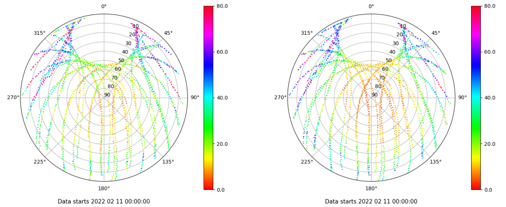
Skyplot for station IBIZ. Parameter M1C Data file IBIZ00ESP_R_2022042.xtr Skyplot for station IBIZ. Parameter M2P Data file IBIZ00ESP_R_2022042.xtr
