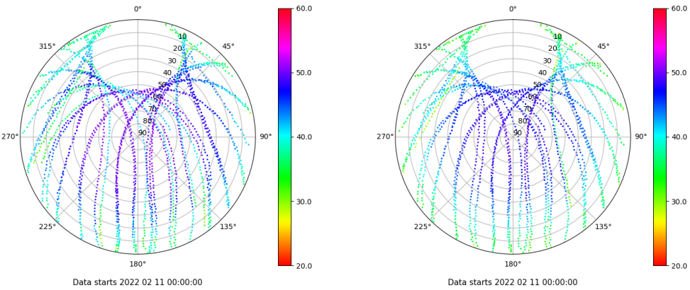
Skyplot for station IBIZ. Signal to Noise S1C Data file IBIZ00ESP_R_2022042.xtr Skyplot for station IBIZ. Signal to Noise S2P Data file IBIZ00ESP_R_2022042.xtr
