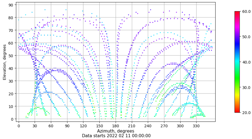
Azimuth-elevation plot for station IBIZ. Signal to Noise S1C Data file IBIZ00ESP_R_2022042.xtr
