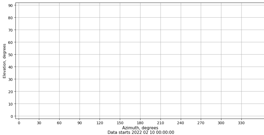
Azimuth-elevation plot for station IBIZ. Signal to Noise S1C Data file IBIZ00ESP_R_2022041.xtr
