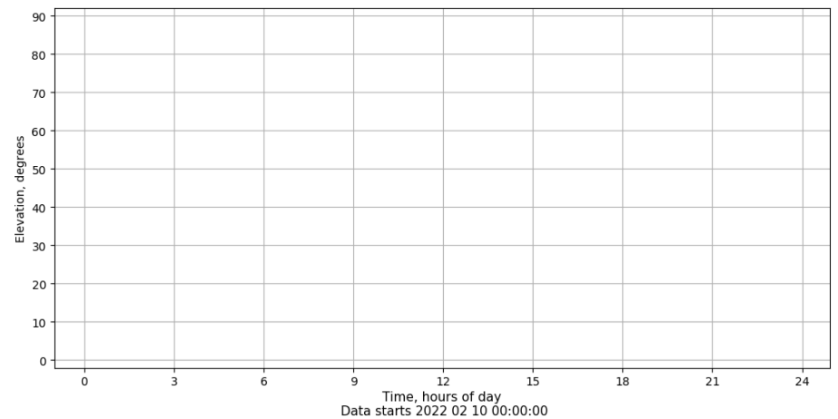
Time-elevation plot for station IBIZ. Signal to Noise S1C Data file IBIZ00ESP_R_2022041.xtr
