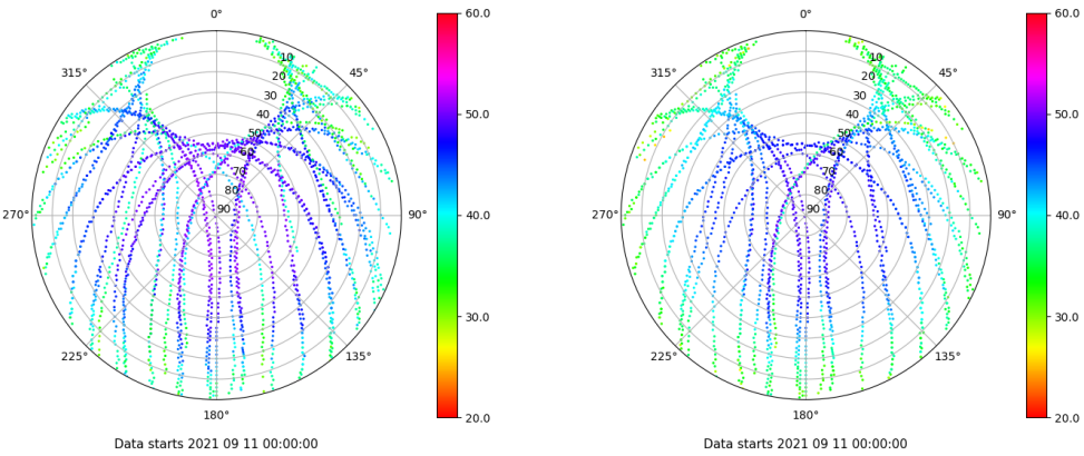
Skyplot for station IBIZ. Signal to Noise S1C Data file IBIZ00ESP_R_2021254.xtr Skyplot for station IBIZ. Signal to Noise S2P Data file IBIZ00ESP_R_2021254.xtr
