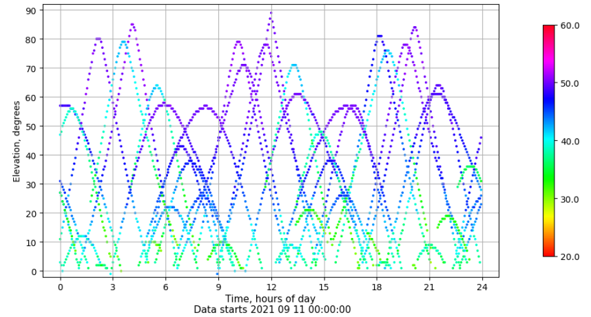
Time-elevation plot for station IBIZ. Signal to Noise S1C Data file IBIZ00ESP_R_2021254.xtr
