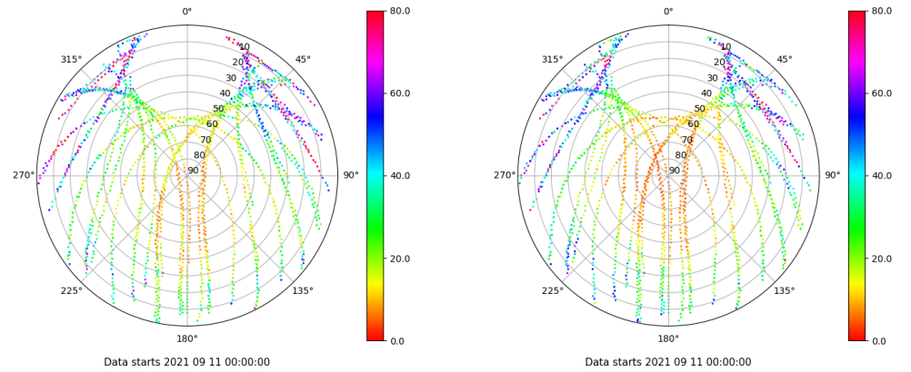
Skyplot for station IBIZ. Parameter M1C Data file IBIZ00ESP_R_2021254.xtr Skyplot for station IBIZ. Parameter M2P Data file IBIZ00ESP_R_2021254.xtr
