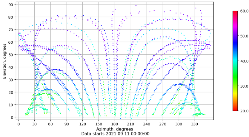
Azimuth-elevation plot for station IBIZ. Signal to Noise S1C Data file IBIZ00ESP_R_2021254.xtr
