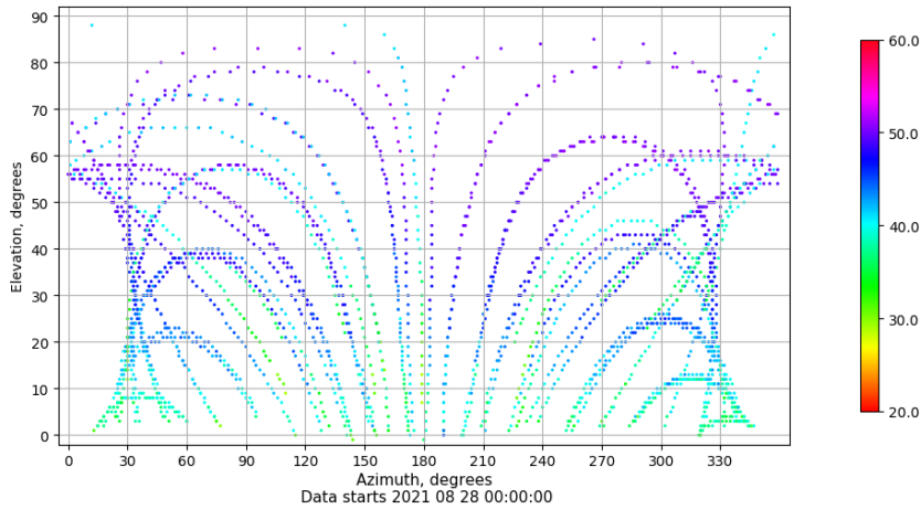
Azimuth-elevation plot for station IBIZ. Signal to Noise S1C Data file IBIZ00ESP_R_2021240.xtr
