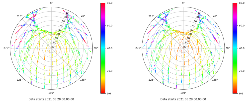
Skyplot for station IBIZ. Parameter M1C Data file IBIZ00ESP_R_2021240.xtr Skyplot for station IBIZ. Parameter M2P Data file IBIZ00ESP_R_2021240.xtr
