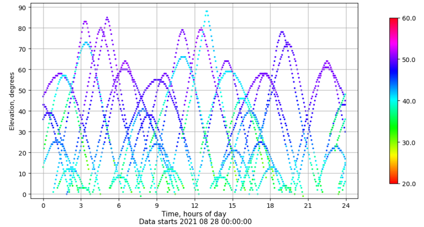
Time-elevation plot for station IBIZ. Signal to Noise S1C Data file IBIZ00ESP_R_2021240.xtr
