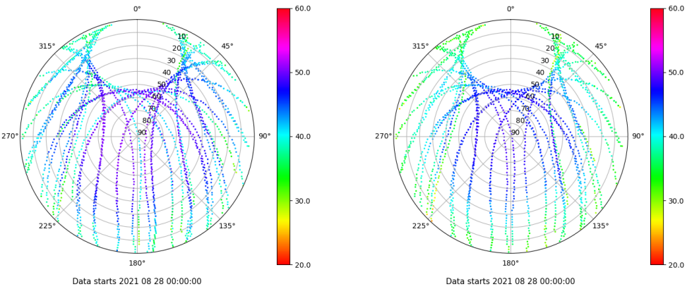
Skyplot for station IBIZ. Signal to Noise S1C Data file IBIZ00ESP_R_2021240.xtr Skyplot for station IBIZ. Signal to Noise S2P Data file IBIZ00ESP_R_2021240.xtr
